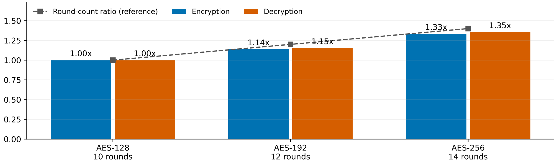
Measured computational cost for 100 MB
