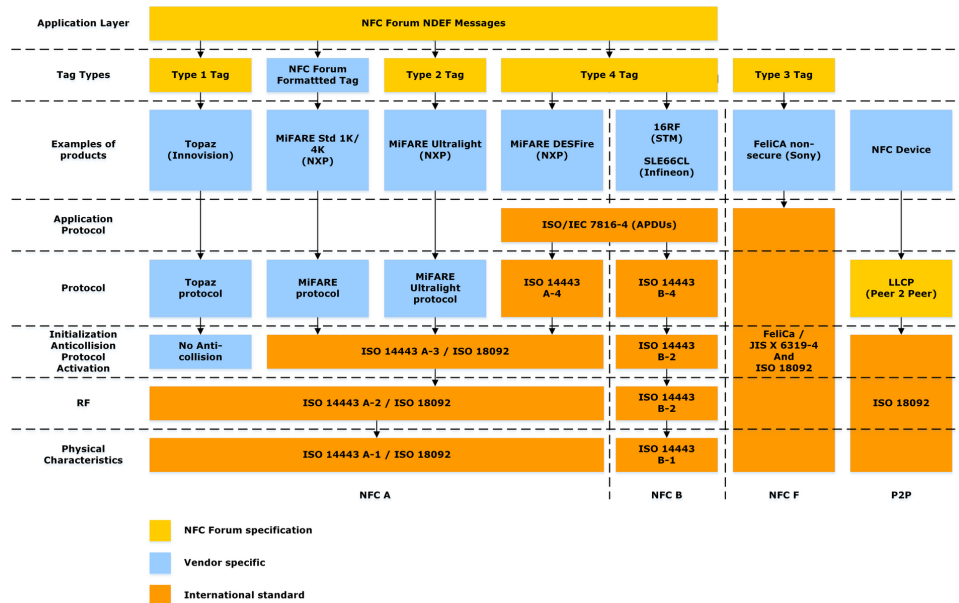
Figure 3.1. NFC Protocol Stack [12]
