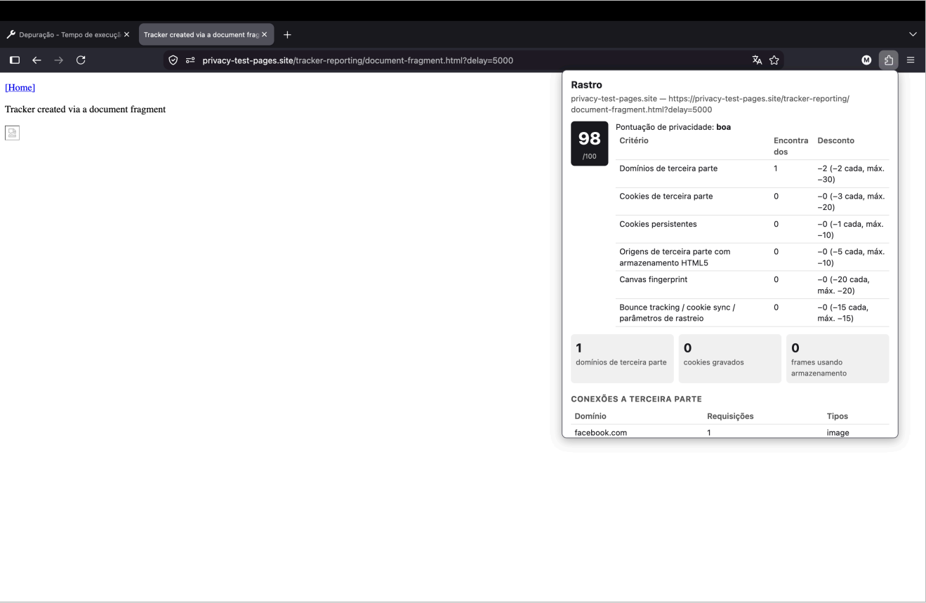
Tracker Reporting — document fragment, delay 5 s
