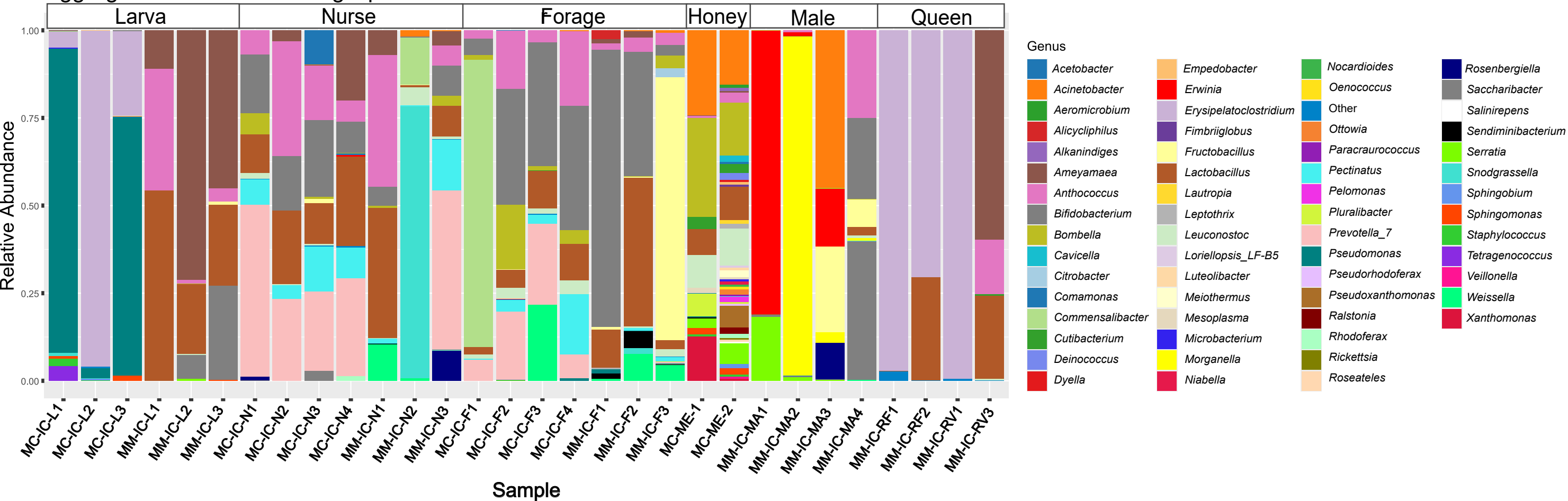
Aggregated Genera Covering Up to 90% Abundance
