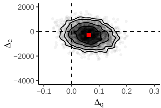
BayesSUR
