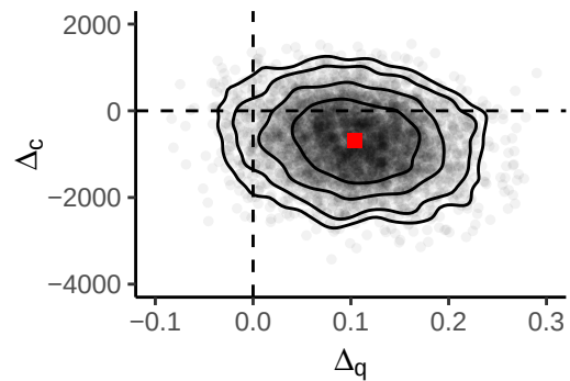
ps-BayesSUR
