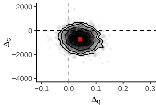
mvBART
