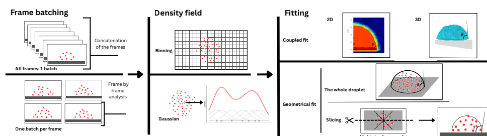
Figure 2: Schematic representation of the composable strategies in wetting-angle-kit to compute contact angle from a MD trajectory.
