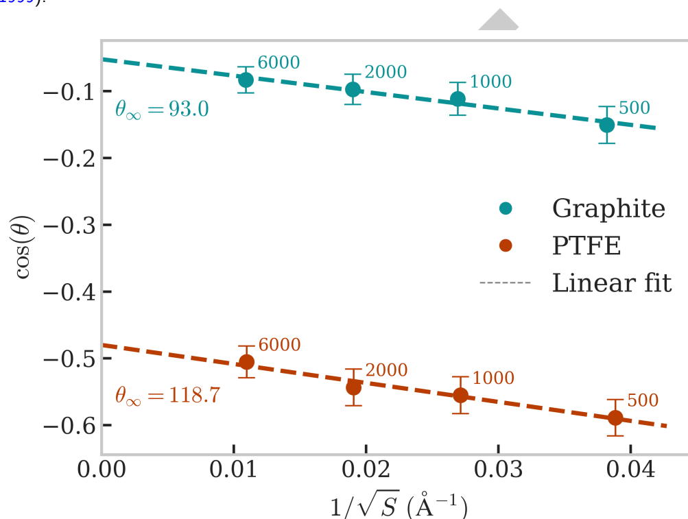
Figure 4: Size-dependent contact angle analysis for water droplets on graphite and PTFE substrates. Values of \cos(\theta) are plotted as a function of the inverse square root of the droplet surface area for droplets containing between 500 and 6000 water molecules. A linear extrapolation following the modified Young's equation is used to estimate the macroscopic (infinite-droplet) contact angle.
