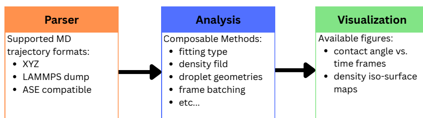
Figure 1: Wetting-angle-kit package structure. The package is composed of three main modules: parsers, analysis, and visualization.
