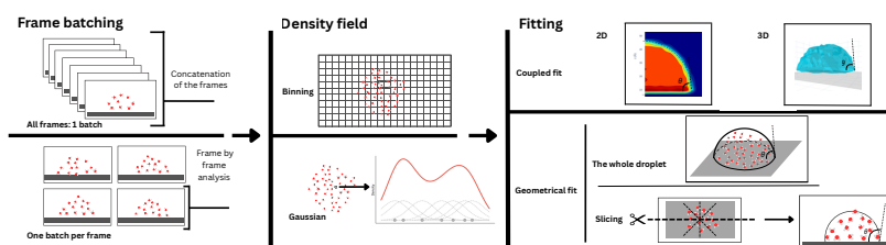
Figure 2: Schematic representation of the composable strategies in wetting-angle-kit to compute contact angle from a MD trajectory.
