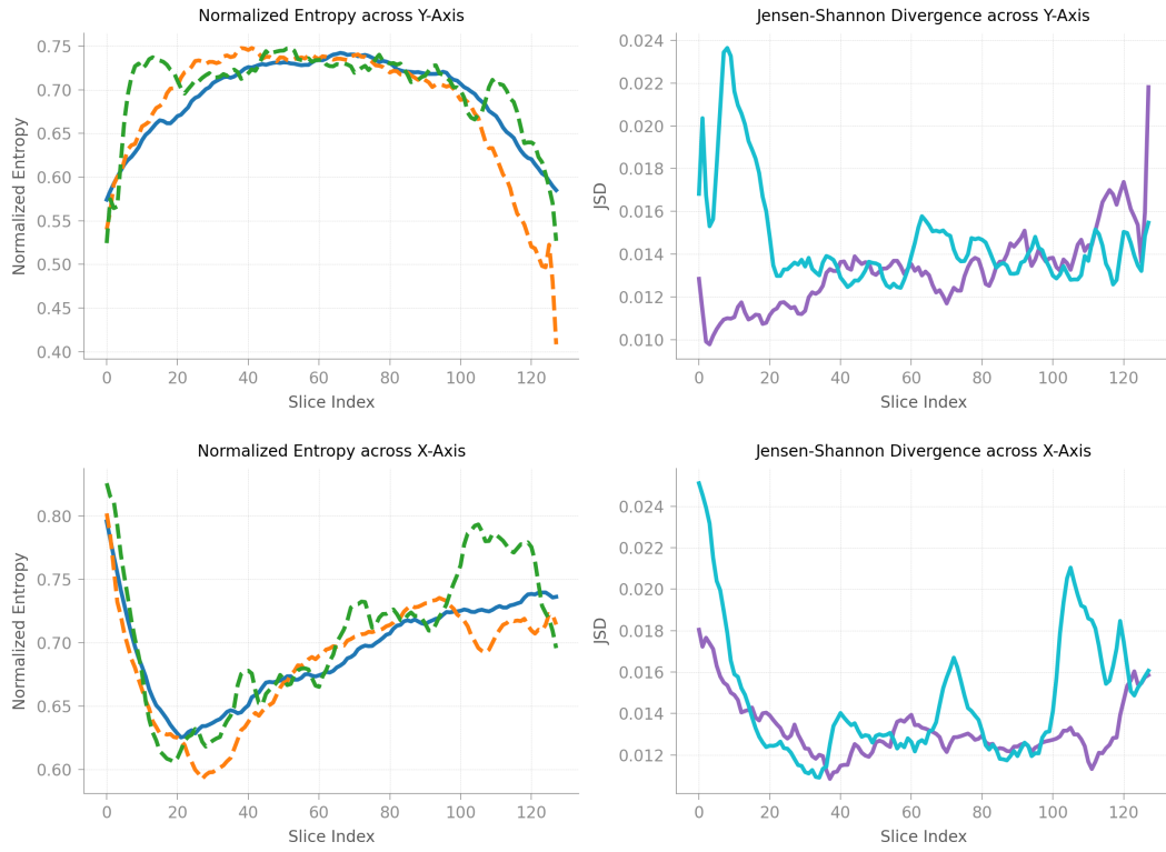
Figure E.1: Comparison of the JSD normalized voxel-wise entropy across the Y, and X axes.
