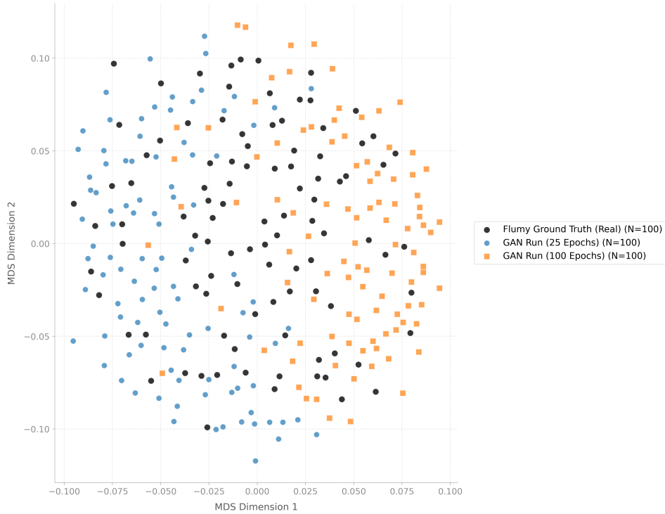
Figure C.2: Multi-Dimensional Scaling (MDS) plot of the MS-SWD values computed for the test dataset, illustrating the distribution shift and clustering behaviour of the model 5 architecture between 25 and 100 training epochs.
