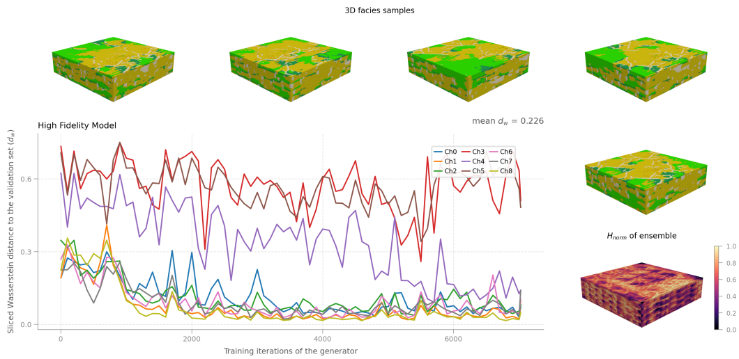
Figure 4.7: Overview of the high-fidelity model metrics and training evolution over 25 epochs.
