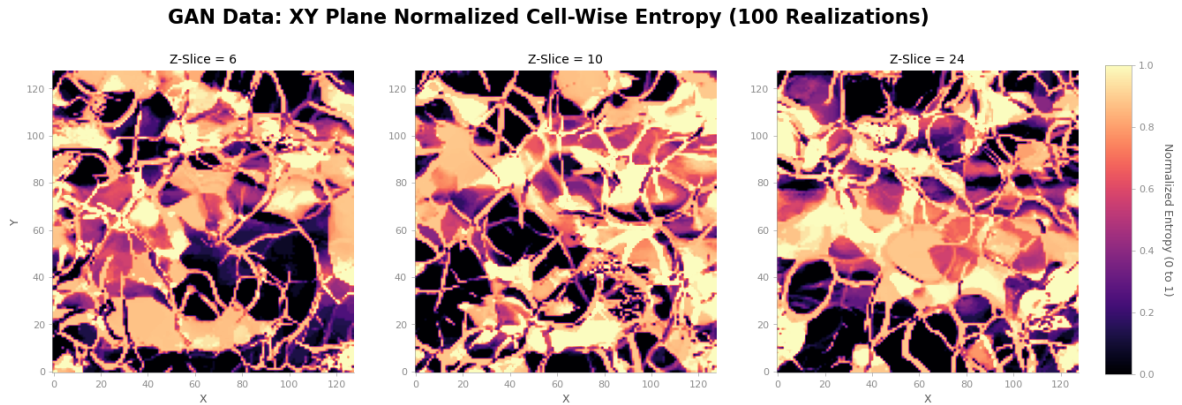
Figure 4.4: Normalized cell-wise spatial entropy across selected horizontal slices ( Z = 6, 10, \text{ and } 24 ) calculated over 100 unconstrained cGAN realizations.
