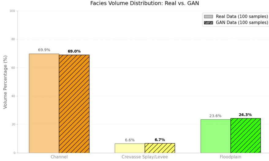
Figure 4.3: Comparative analysis of global facies volume percentages between the true training dataset and 100 unconstrained cGAN realizations, demonstrating macro-scale categorical matching.
