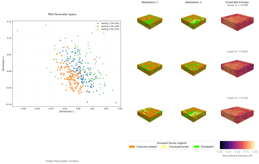
Figure 4.1: MDS plot with two 3D facies samples displayed and a 3D pixel-wise entropy per setting.
