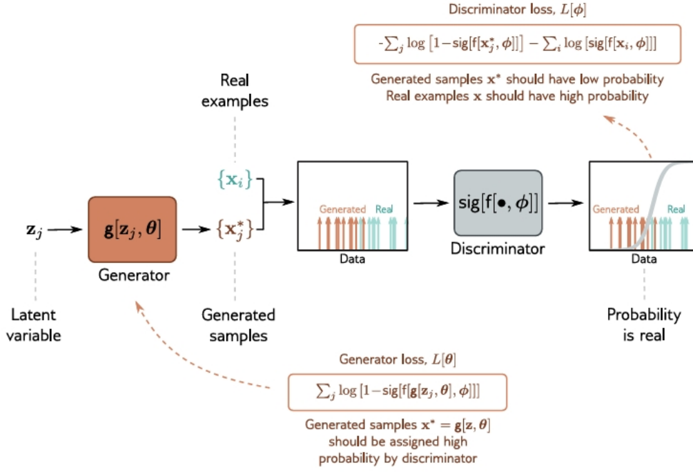
Figure 2.5: Basic overview of a standard GAN architecture with a Generator, constructing fake samples from a random latent variable z_j and a Discriminator deciding which of the two samples is the real sample (Prince, 2023).
