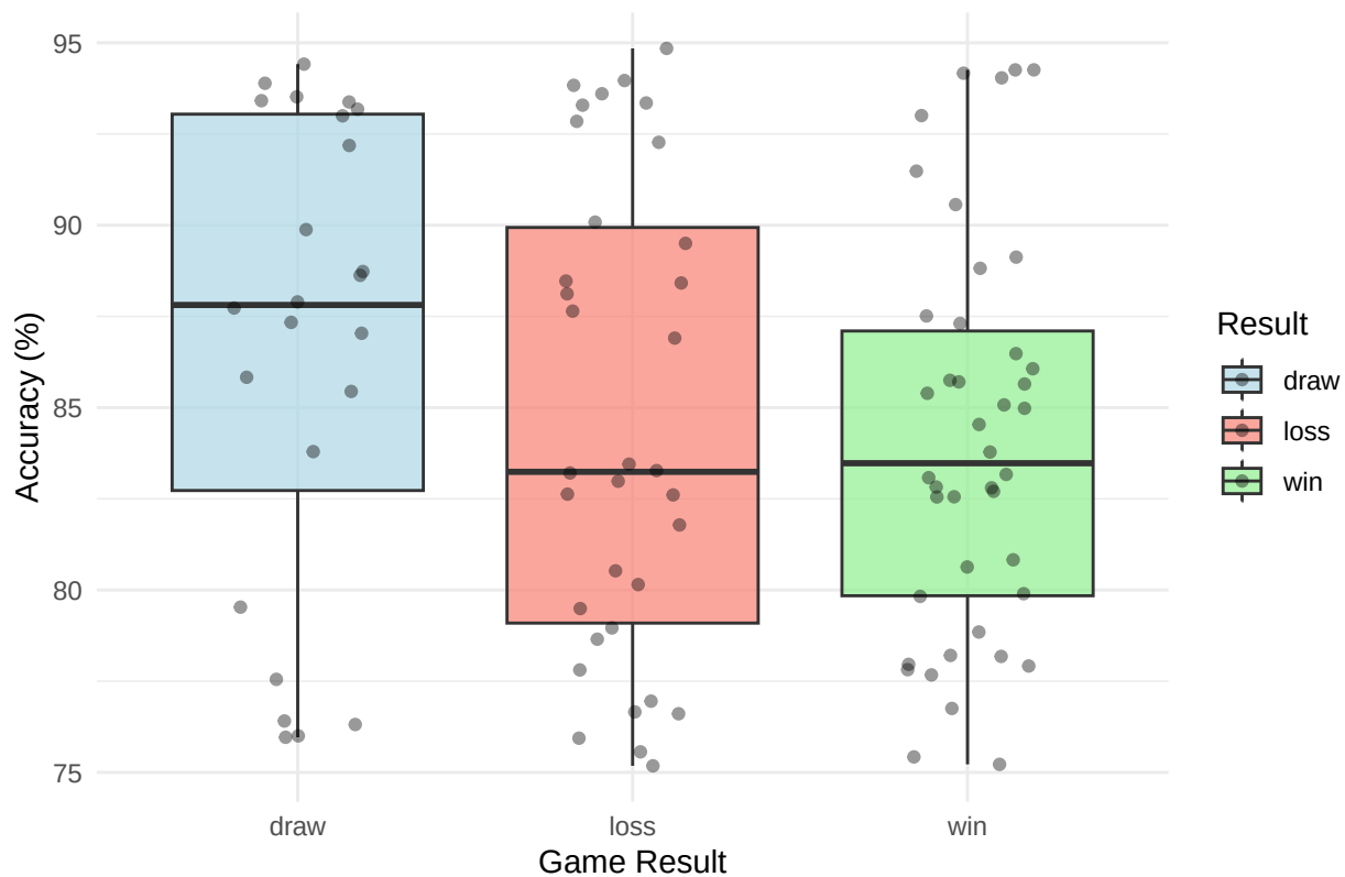
Accuracy Distribution by Game Outcome
