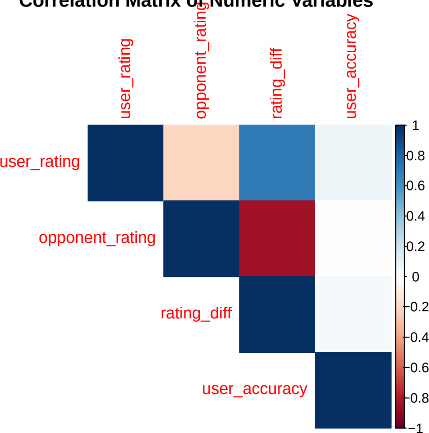
Correlation Matrix of Numeric Variables
