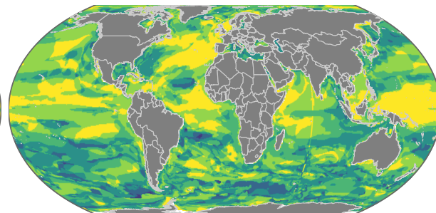
Large Zooplankton
