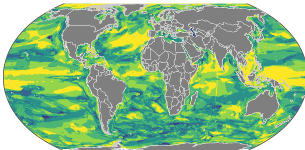
Small Zooplankton
