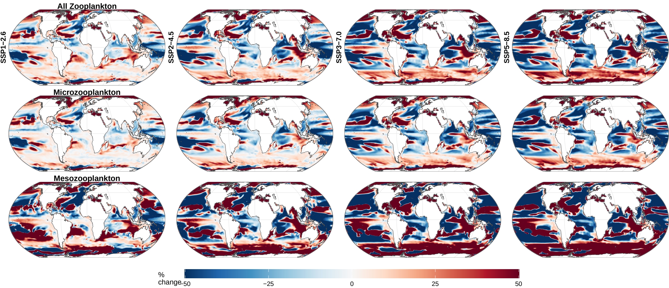
CanESM5-CanOE - % Change in Zooplankton Biomass (1993-2014 to 2081-2100)
