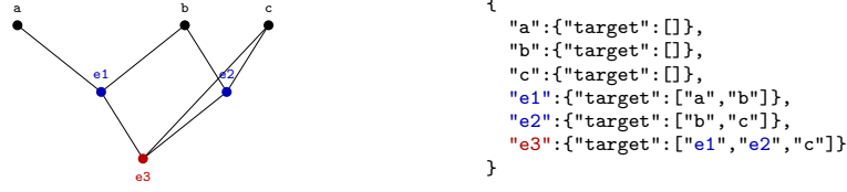
Figure 2: HyperGraphDB data model: every entity is an atom with a target set. Black = atoms (target = [] ), blue = hyperedges, red = higher-order hyperedge ( e_3 references e_1 and e_2 ).
