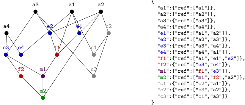
Figure 5: Stage coloring of the same network: black = stage 0 (atoms), blue = stage 1, red = stage 2, purple = stage 3, green = stage 4, gray = cycle (no finite stage). Entries e1 and f2 both have degree 1, but belong to different stages: e1 enters at stage 1 (all refs are atoms), f2 at stage 2 (refs include e3 from stage 1).
