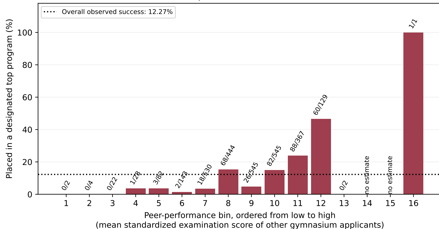
Equal-width bins (16)
