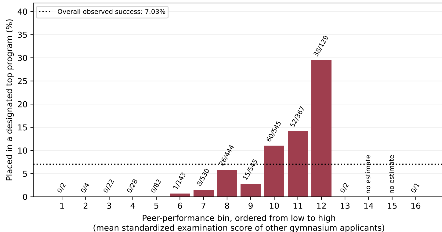
Equal-width bins (16)
