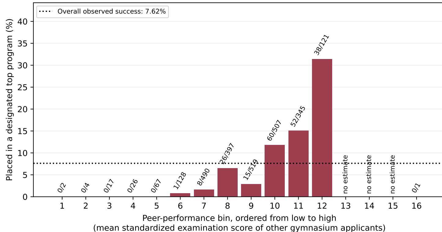
Equal-width bins (16)
