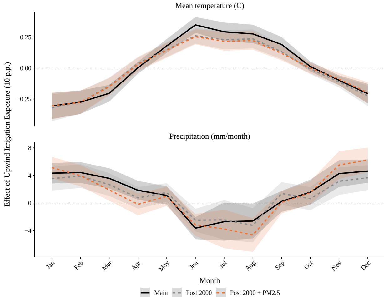
Figure A25: Climate Results controlling for PM 2.5
