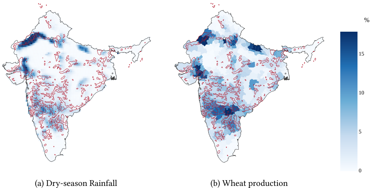
Figure 4: Projected effects of canal irrigation schemes under construction
