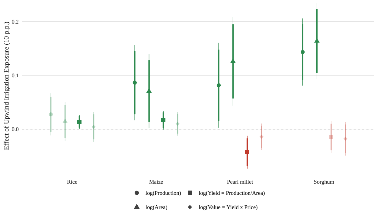
Figure 5: Effect of Upwind Irrigation by Crop
