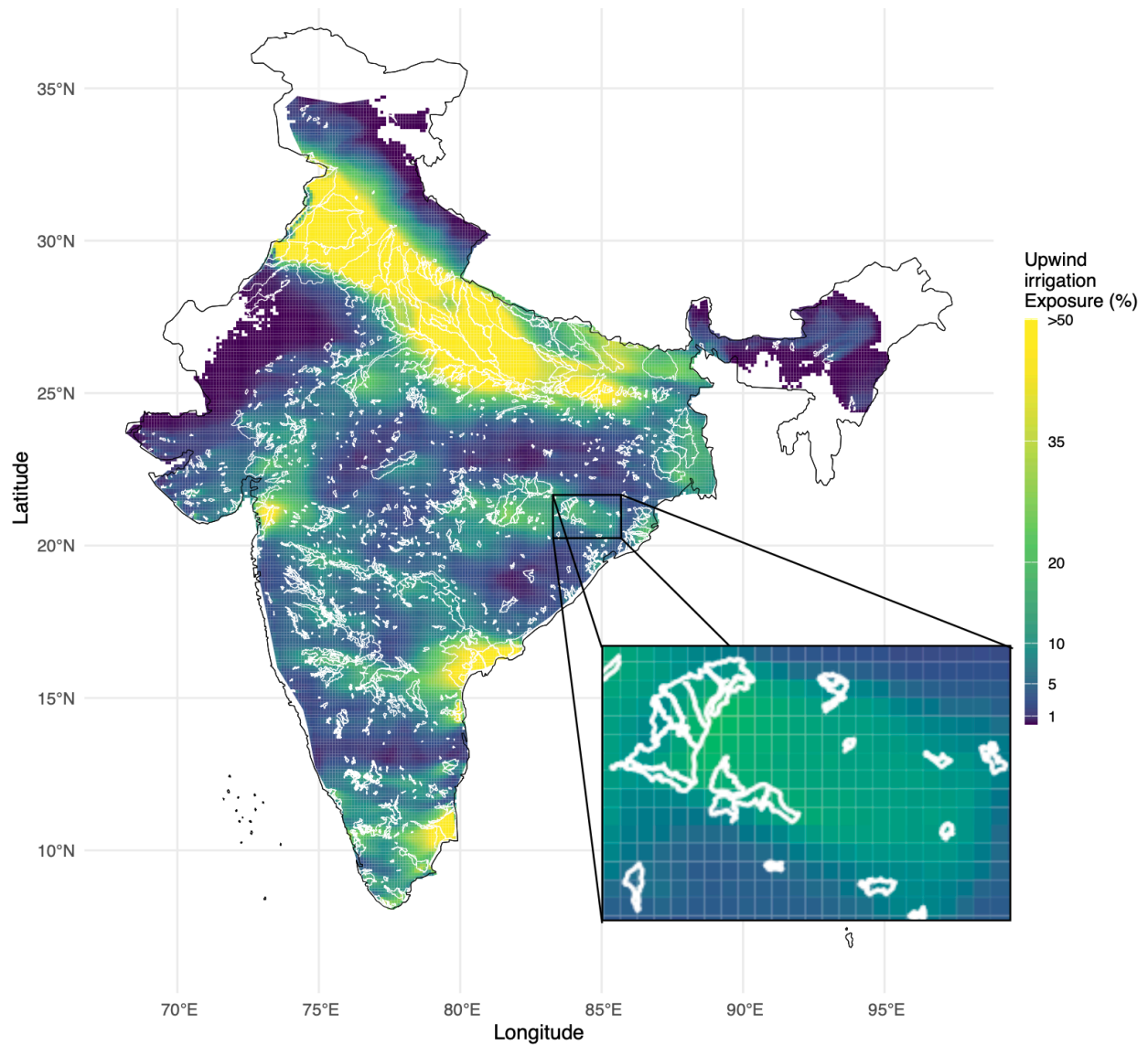
Figure 2: Average Upwind Irrigation Exposure Across India (1966-2020)
