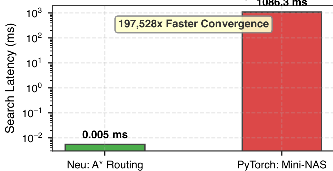
(c) Architectural Pathfinding Latency
