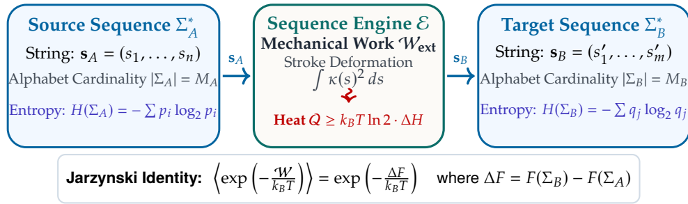
Figure 1: The Thermodynamic Cycle of Sequence Transformation: processing symbolic strings from alphabet \Sigma_A to alphabet \Sigma_B expends stroke curvature energy \int \kappa(s)^2 ds , performs work \mathcal{W} , and dissipates Landauer heat Q_{\text{diss}} into the physical substrate.
