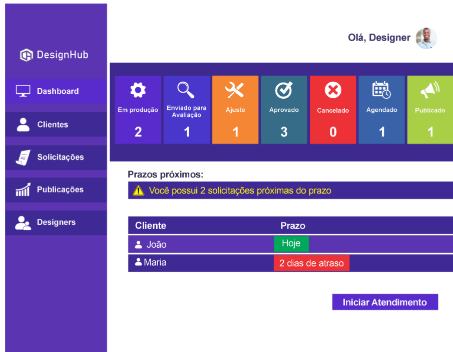
FIGURA 7 – Dashboard Inicial
