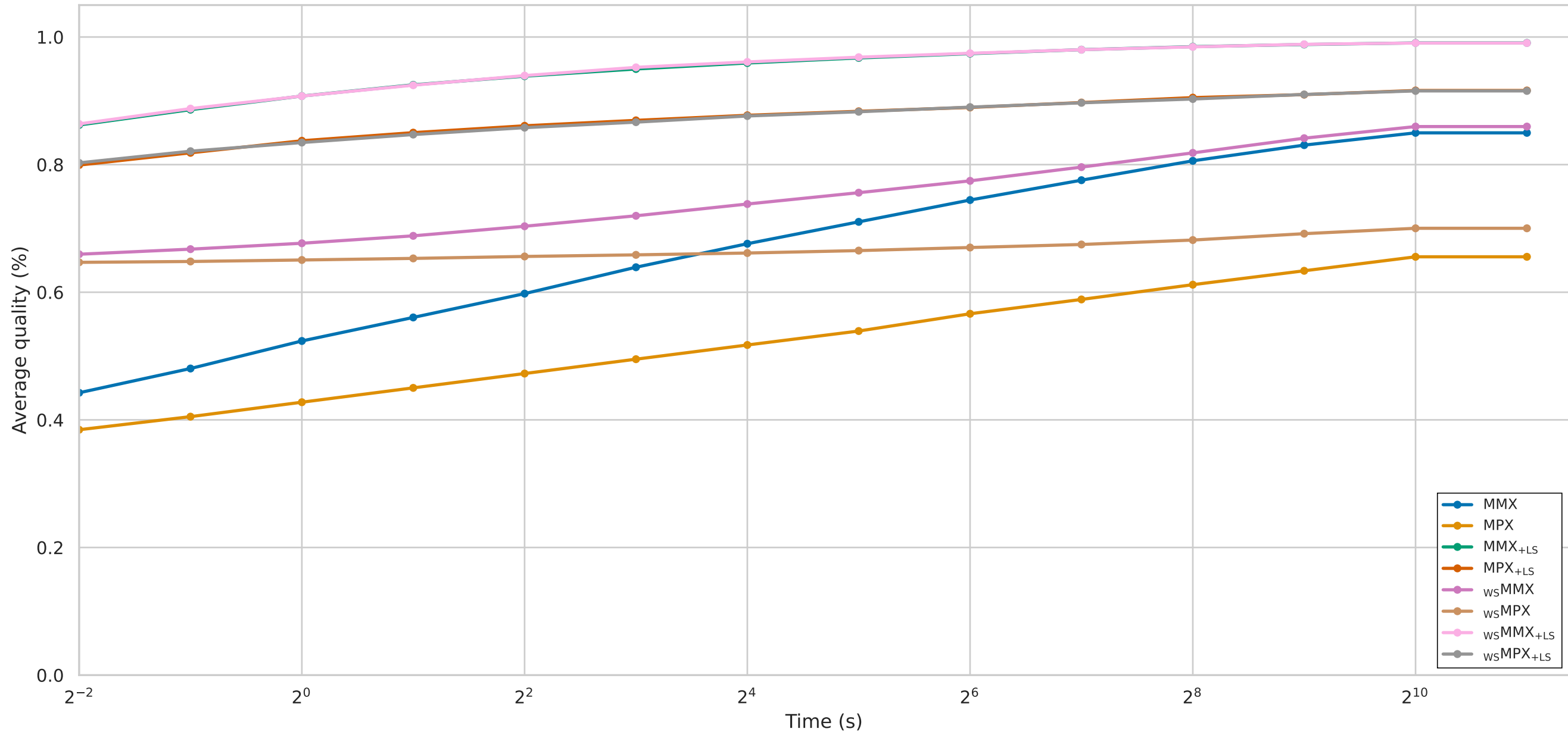
Average performance over time by configuration group
