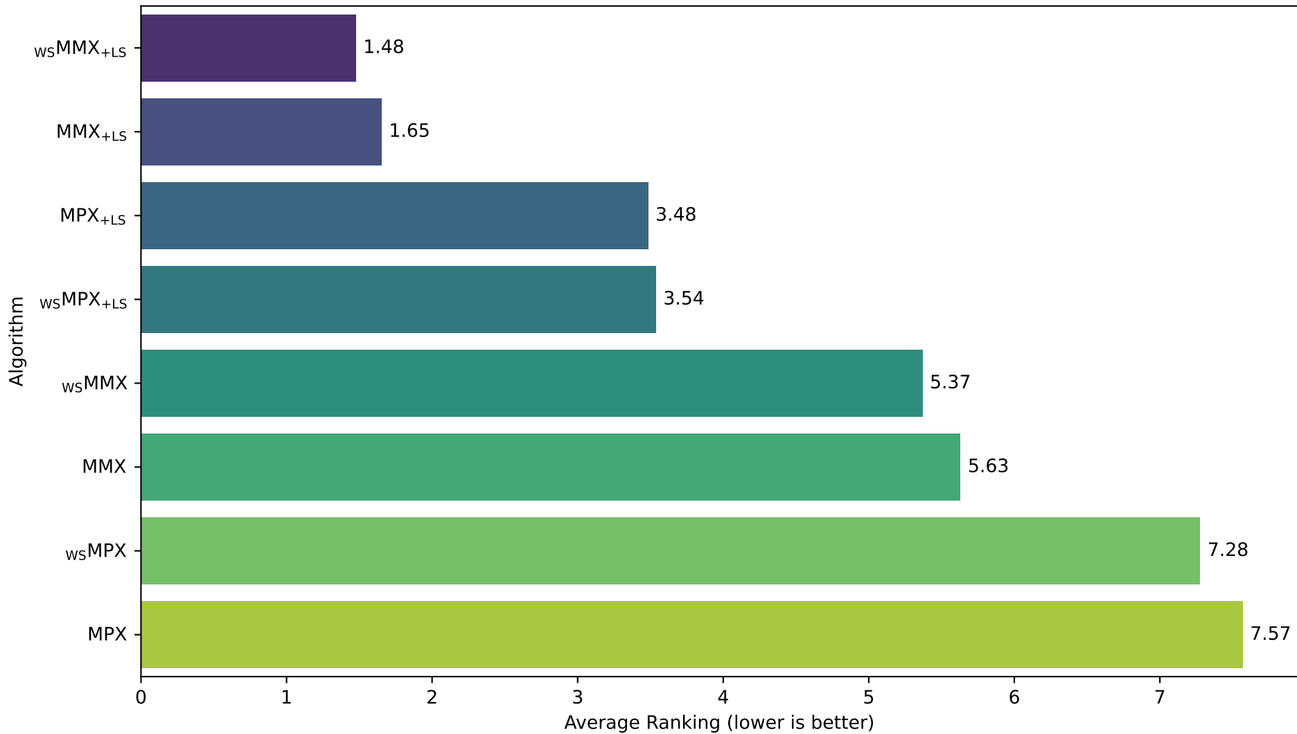
Average Ranking of Algorithms (Friedman)
