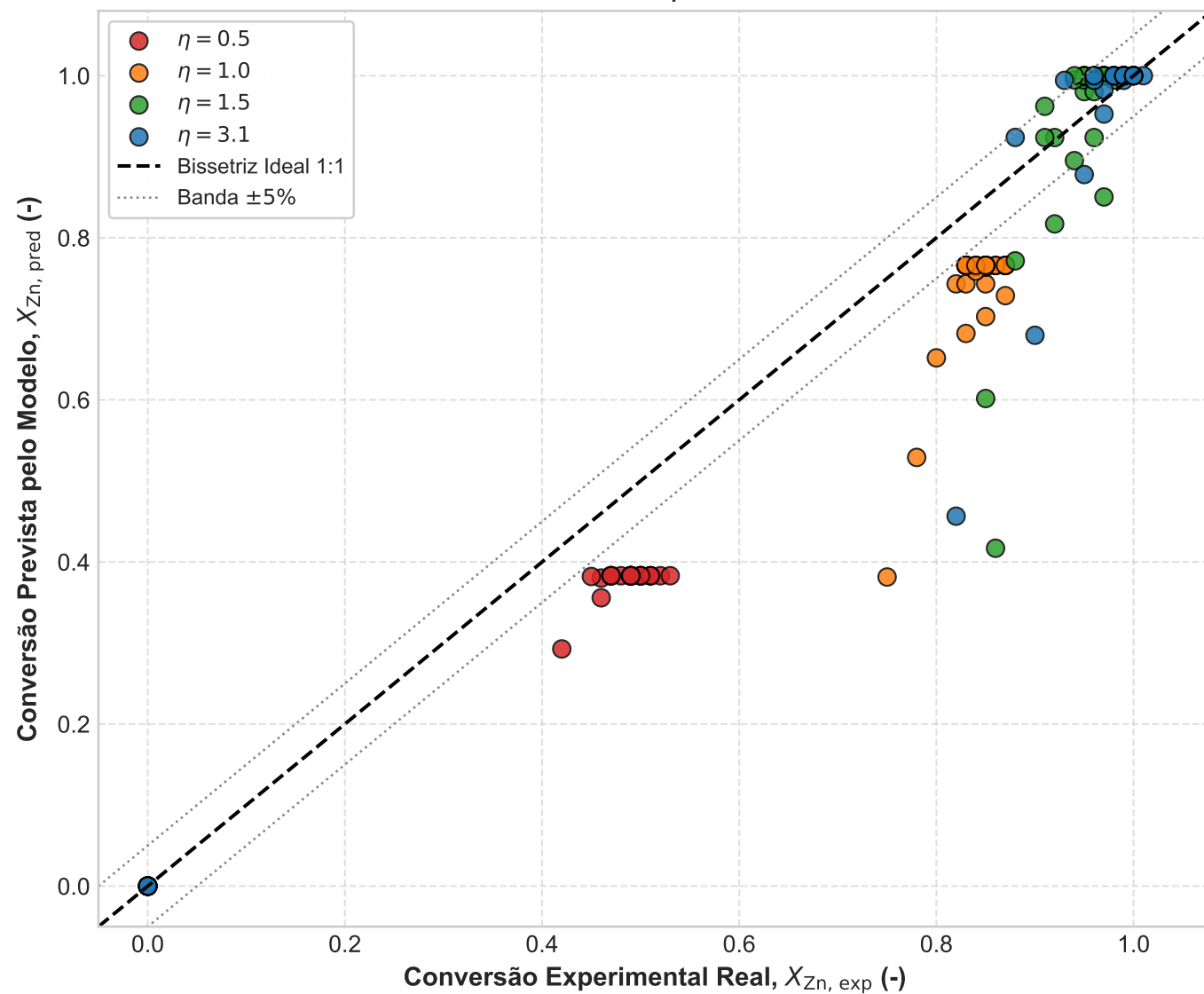
Painel (a) — Modelo Mecanístico Nominal ( \alpha=5500 \mu\text{m}/\text{min} )
