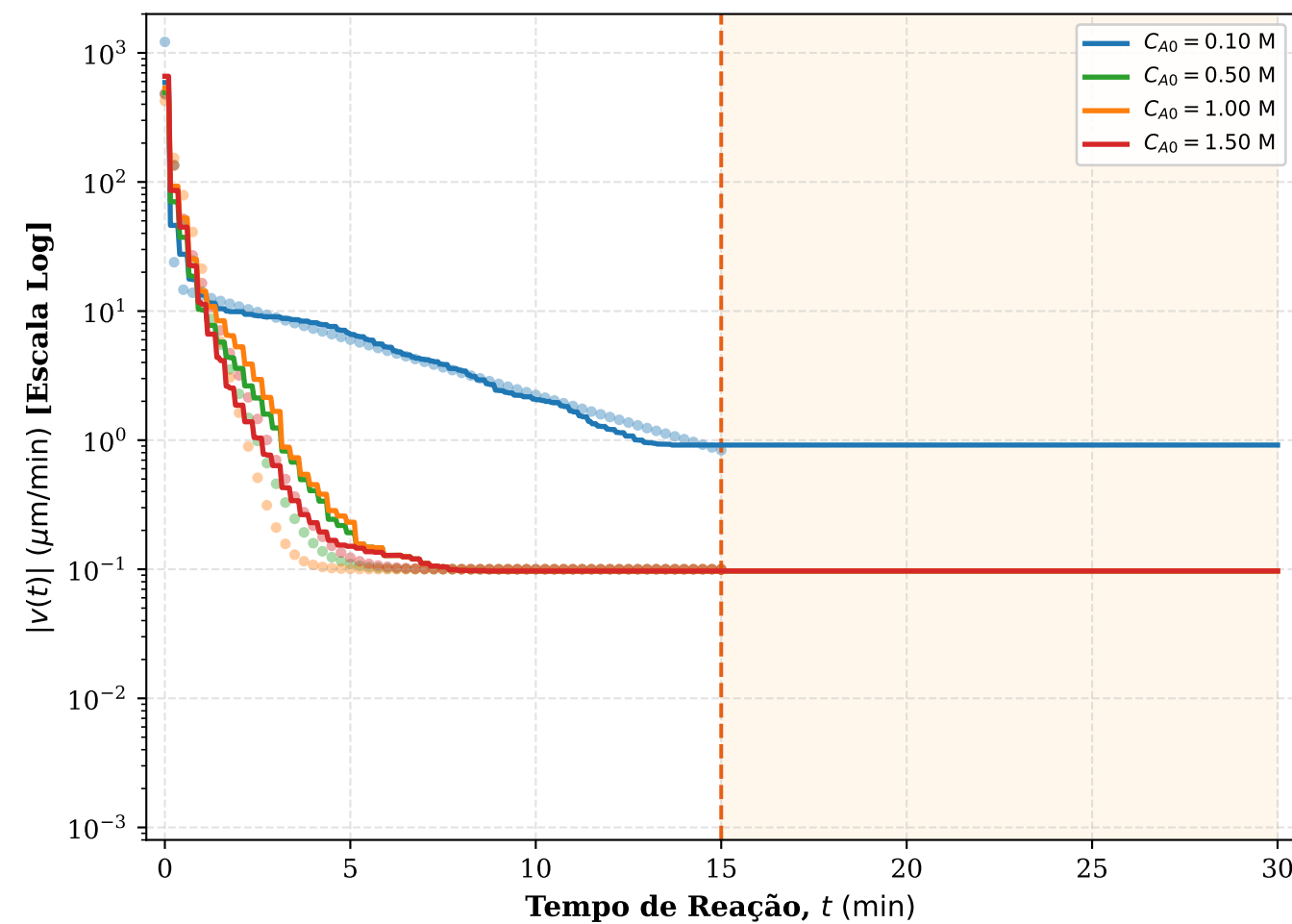
Painel (c) — Razão Molar \eta = 1.5
