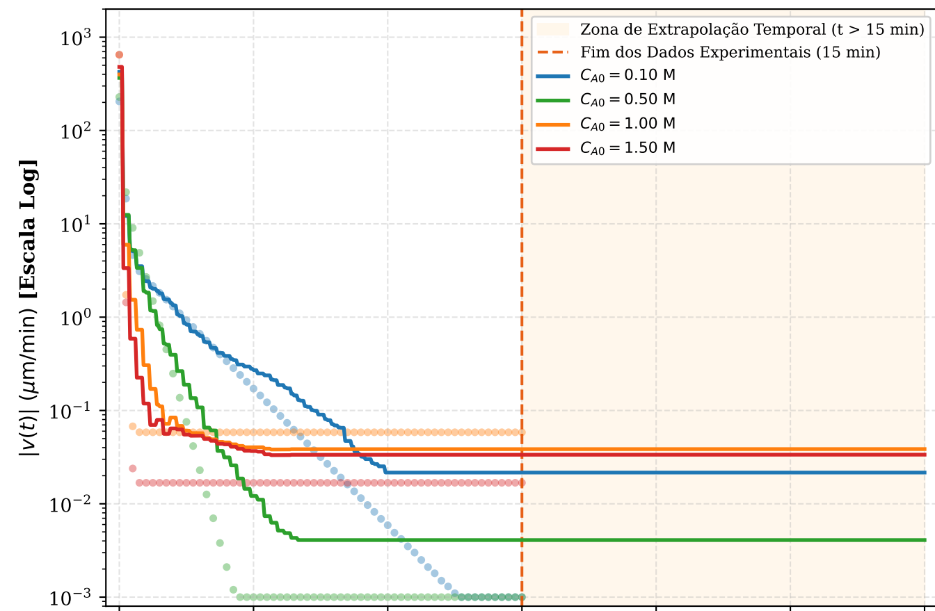
Painel (c) — Razão Molar \eta = 1.5
