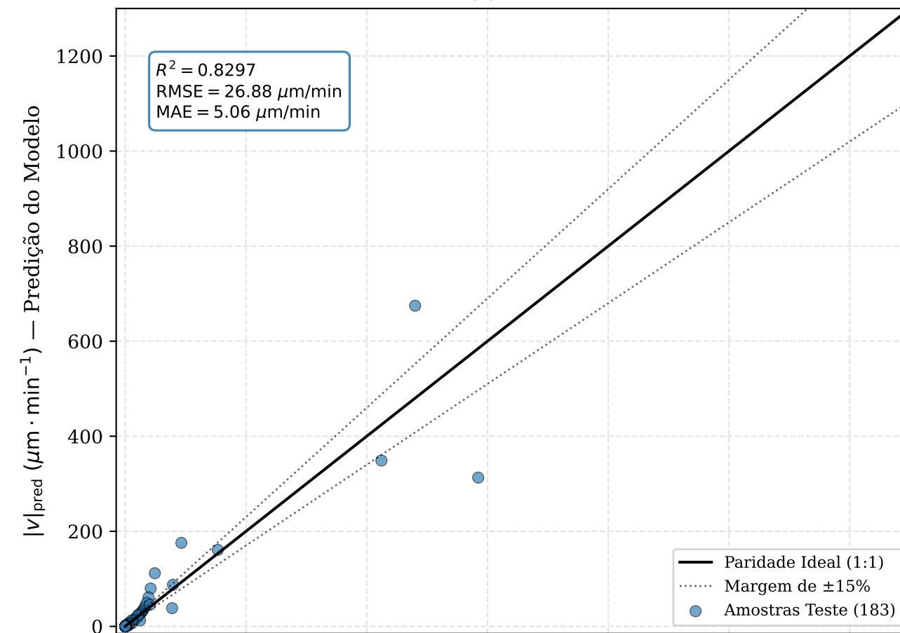
(c) SVR
