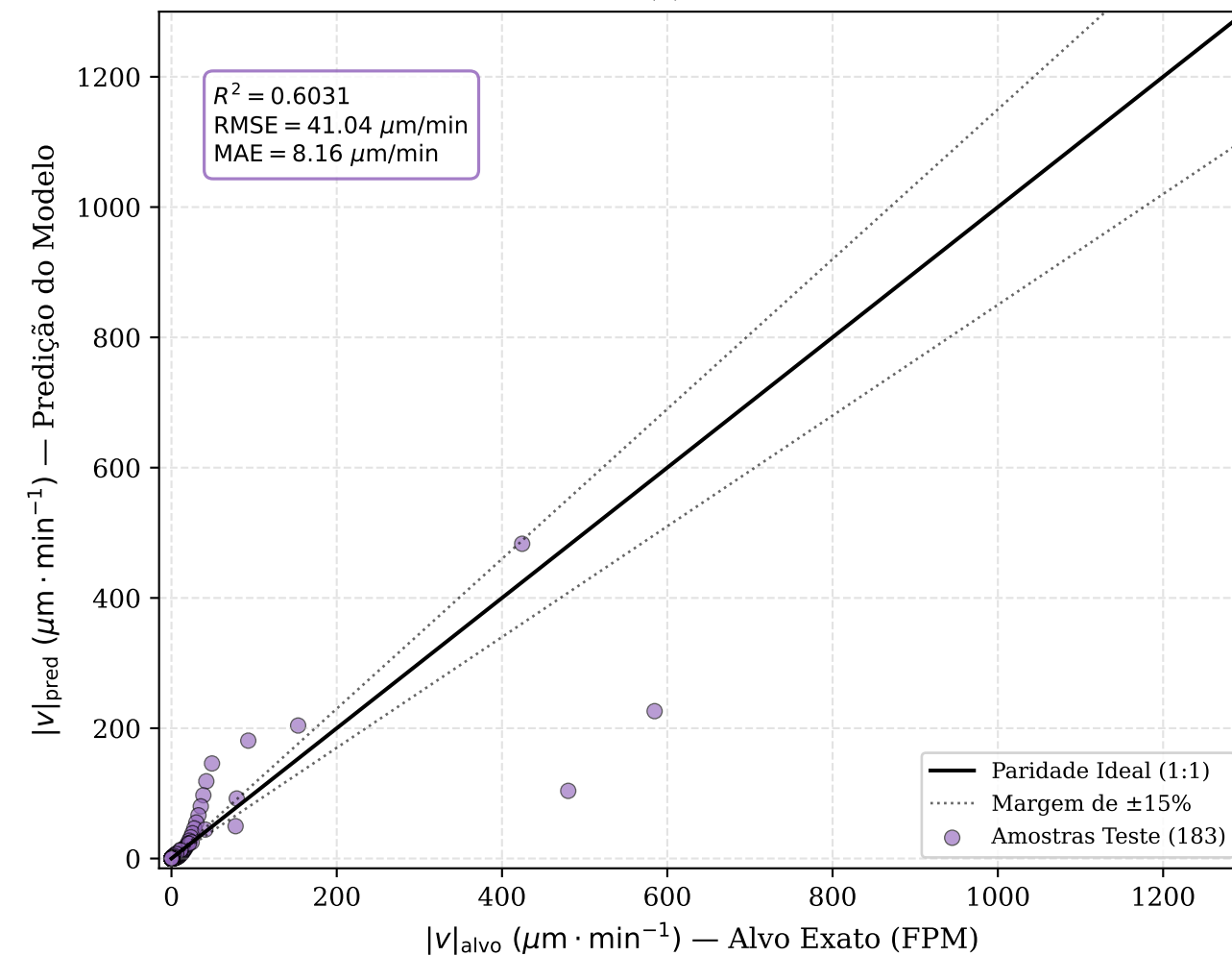
(c) SVR
