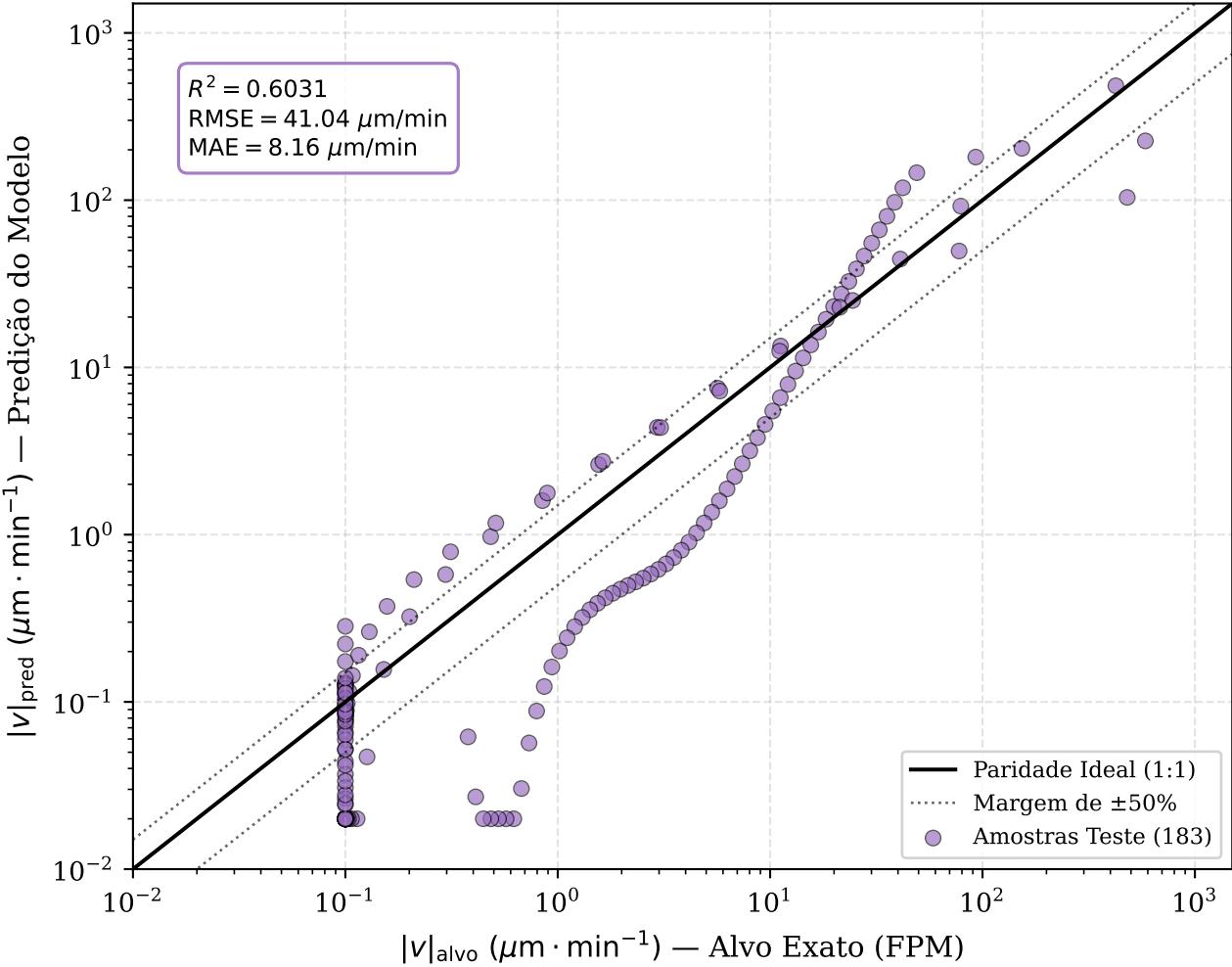
(c) SVR
