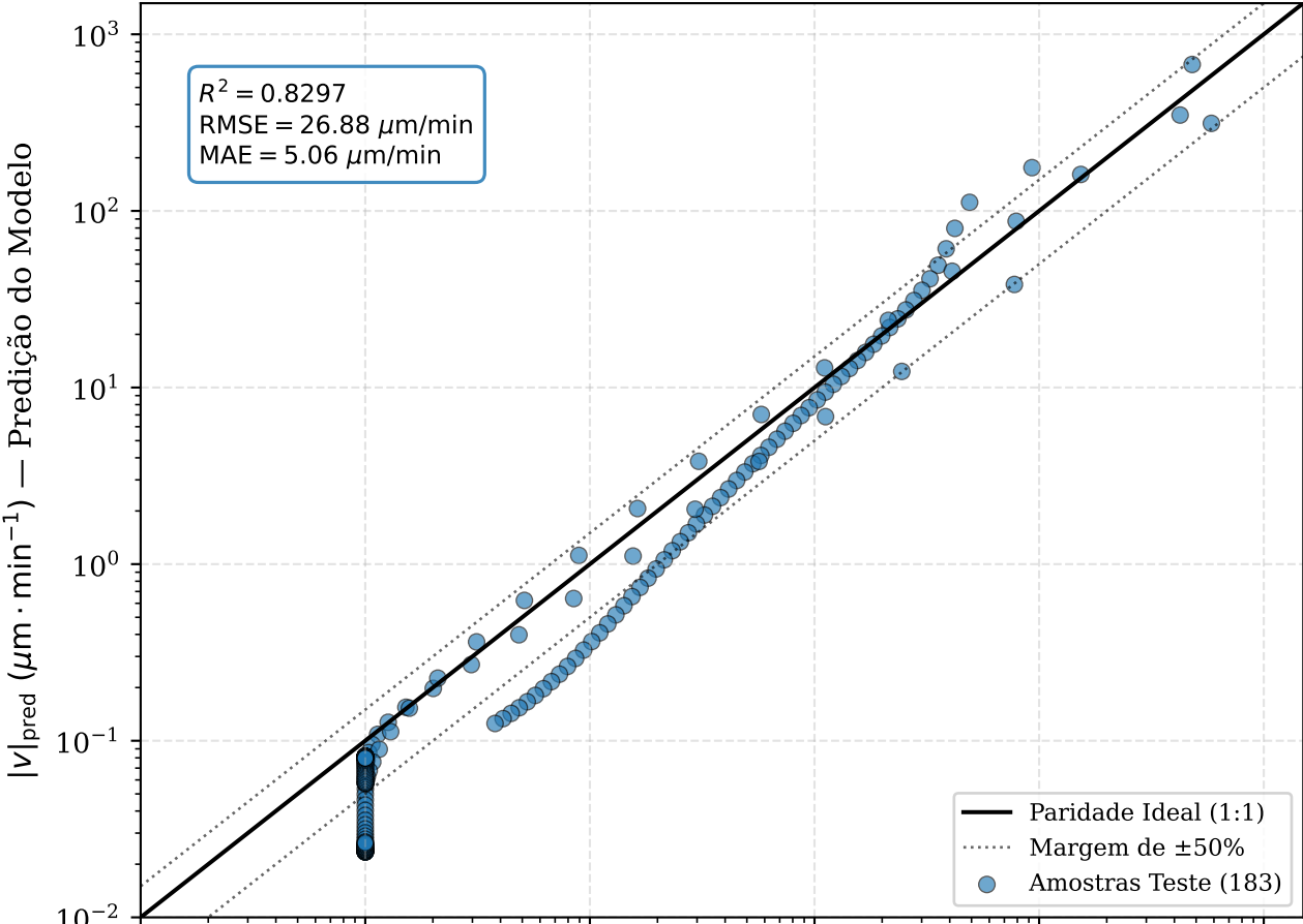
(a) MLP
