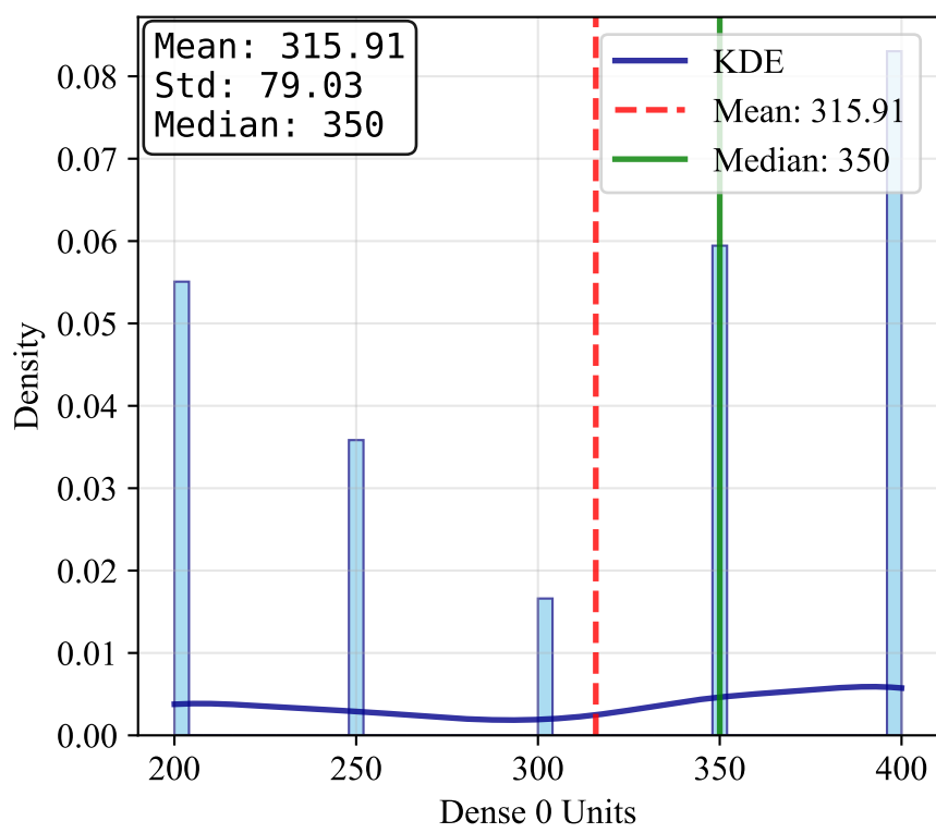
Dense 0 Units
