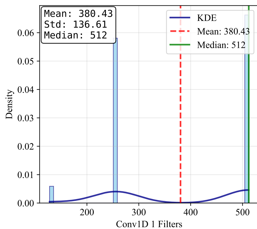
Conv1D 1 Filters
