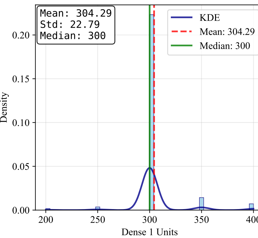
Dense 1 Units
