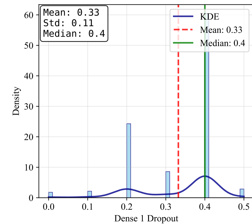
Dense 1 Dropout
