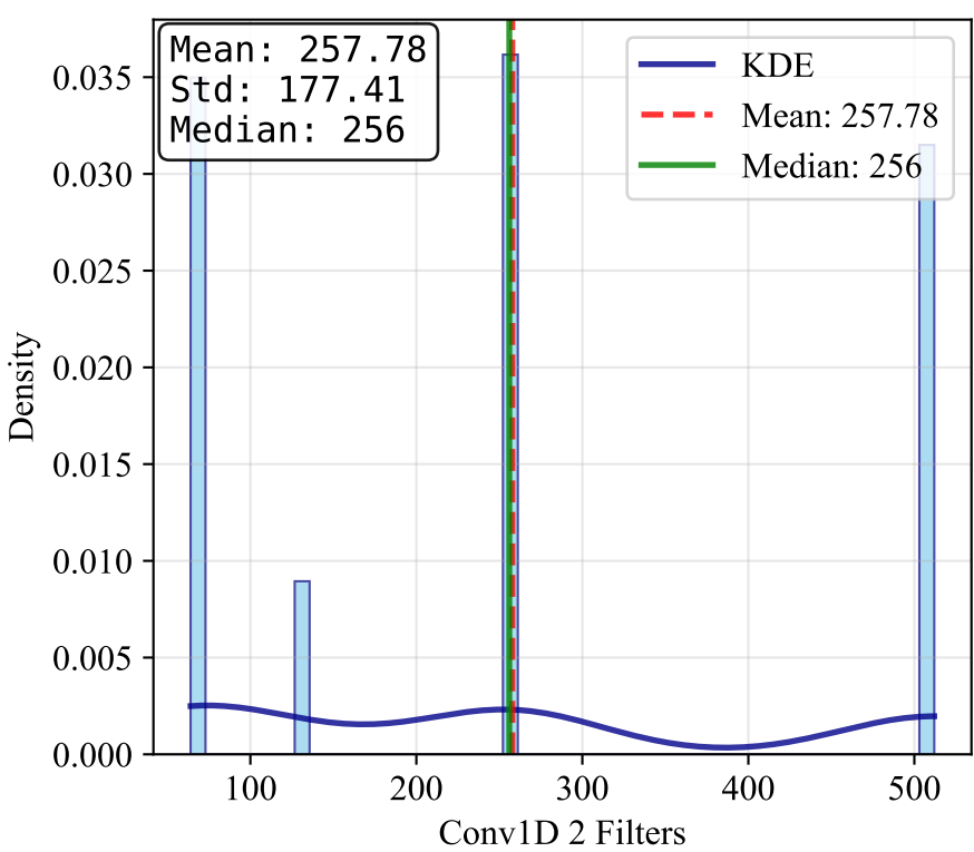
Conv1D 2 Filters
