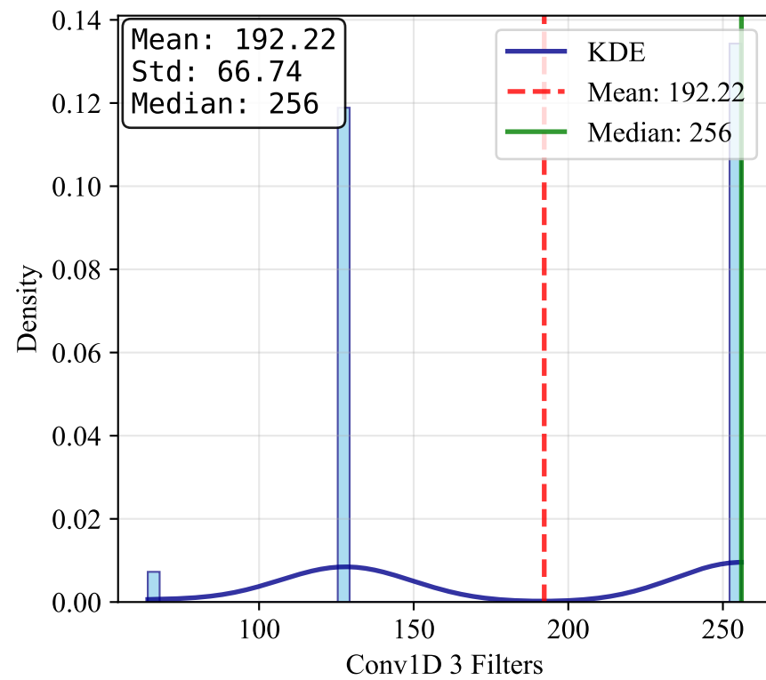
Conv1D 3 Filters
