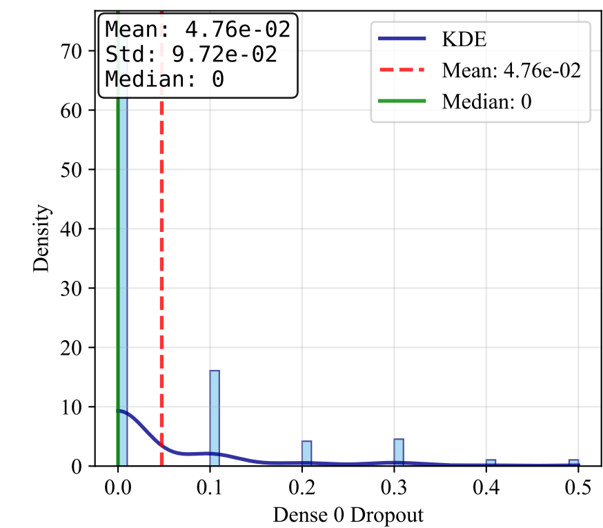
Dense 0 Dropout
