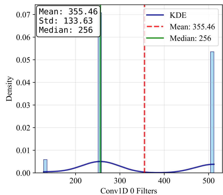
Conv1D 0 Filters
