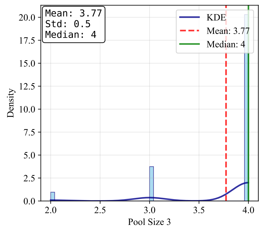
Pool Size 3
