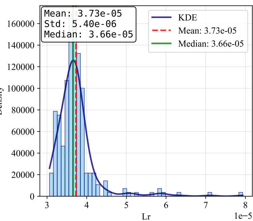
Lr
