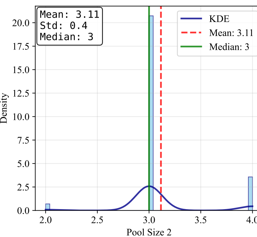
Pool Size 2
