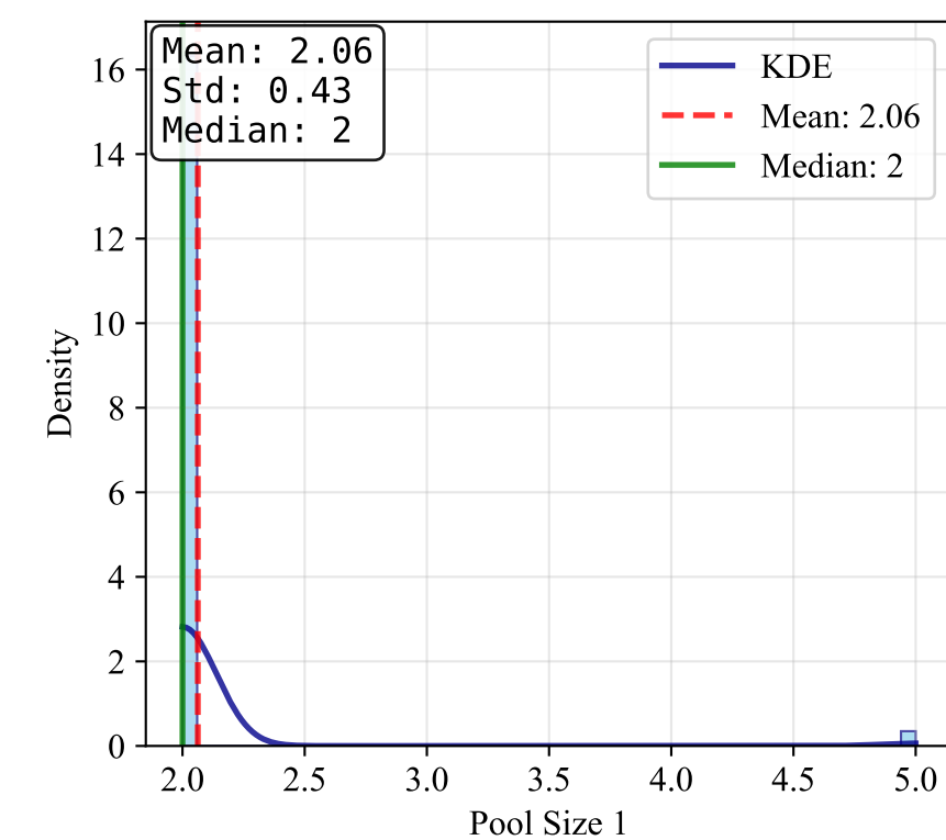
Pool Size 1
