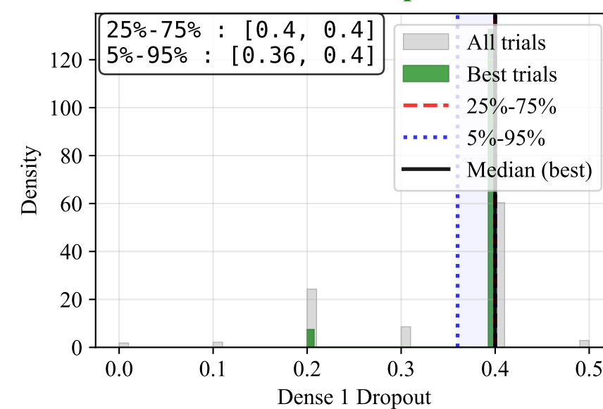
Dense 1 Dropout
