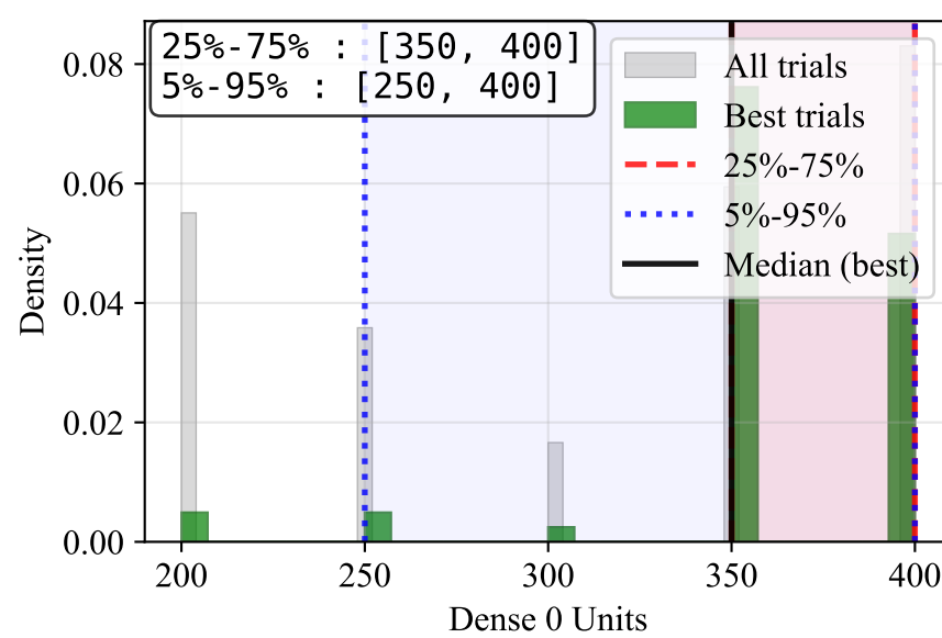
Dense 0 Units
