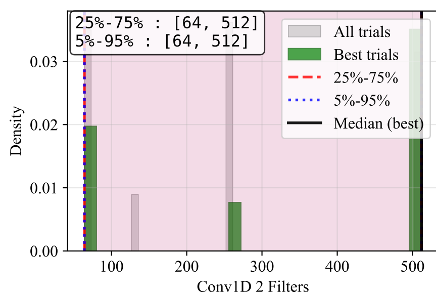
Conv1D 2 Filters
