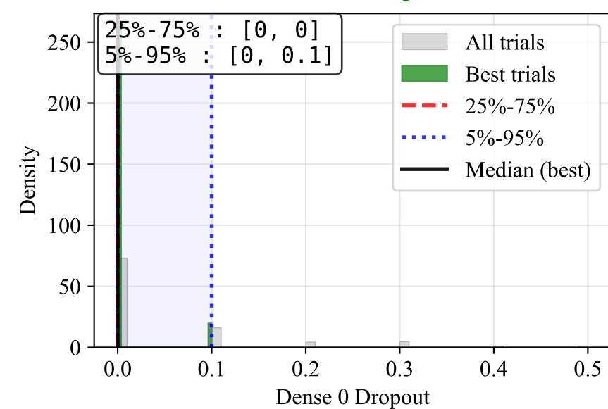
Dense 0 Dropout
