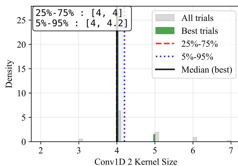
Conv1D 2 Kernel Size
