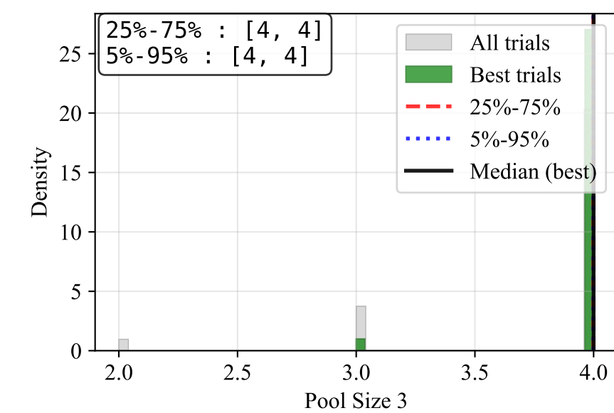
Pool Size 3
