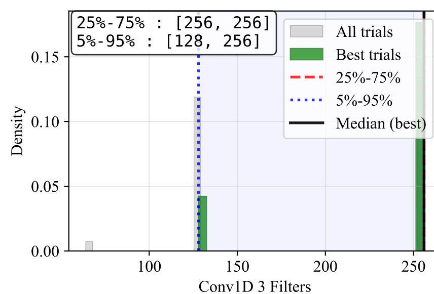
Conv1D 3 Filters
