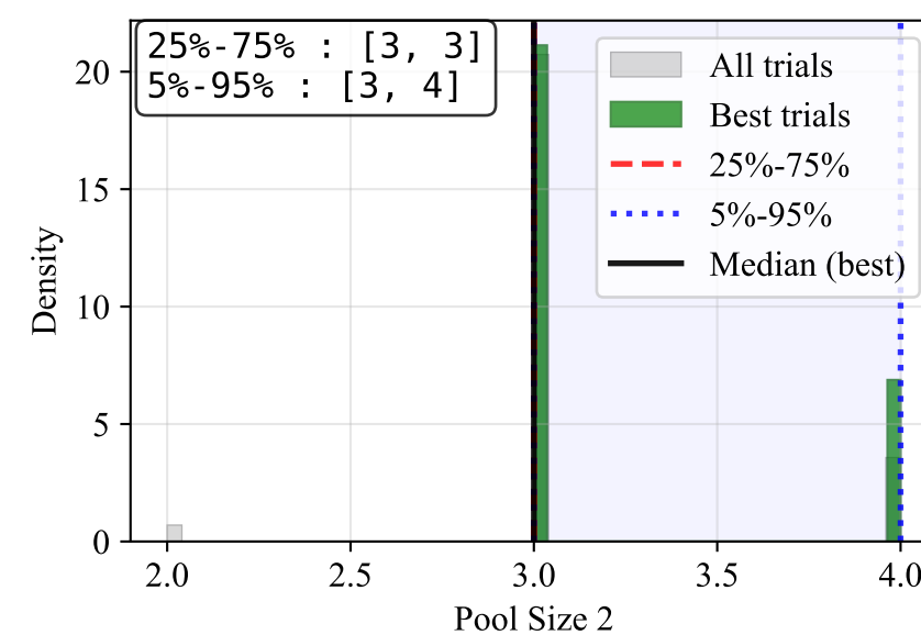
Pool Size 2
