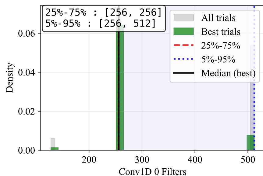
Conv1D 0 Filters
