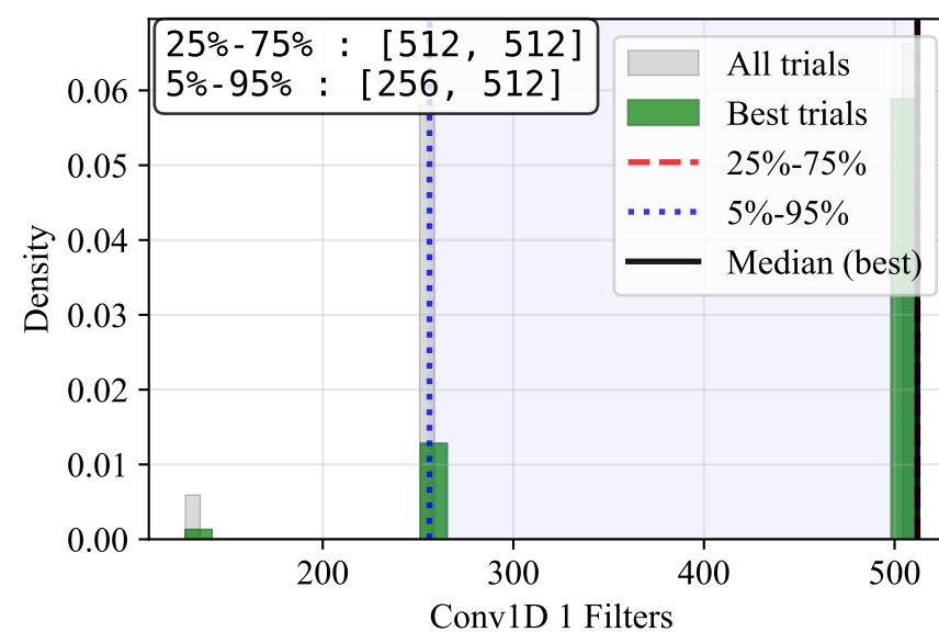
Conv1D 1 Filters
