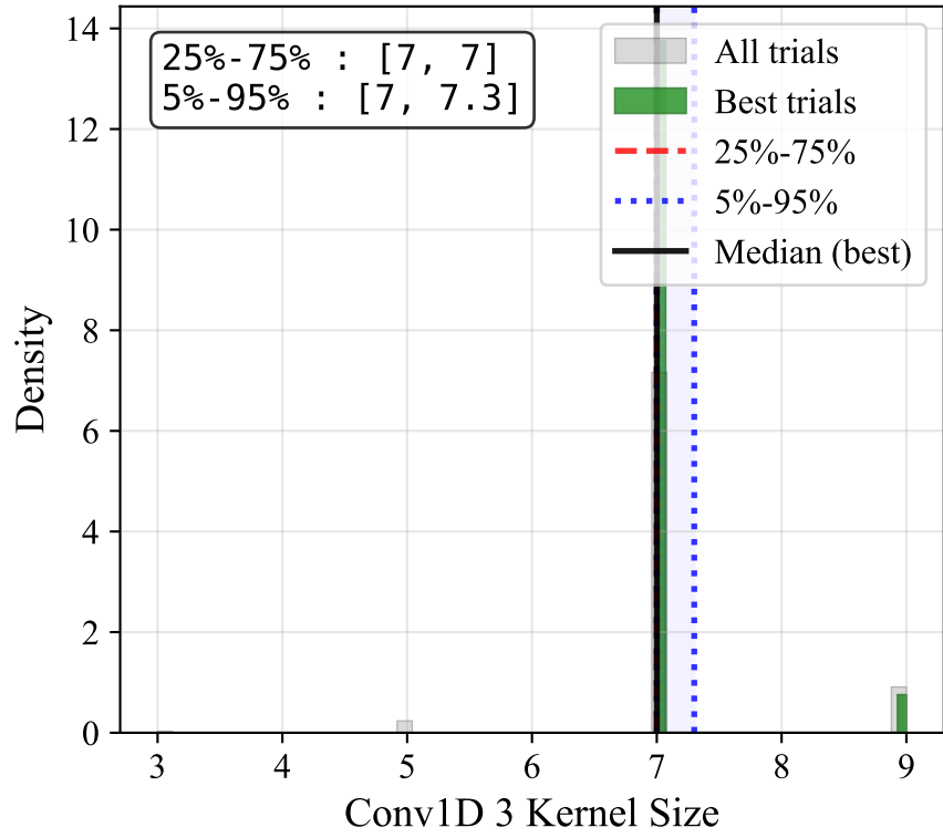
Conv1D 3 Kernel Size
