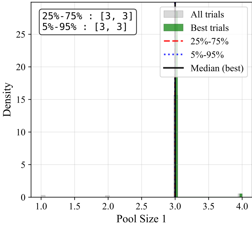
Pool Size 1
