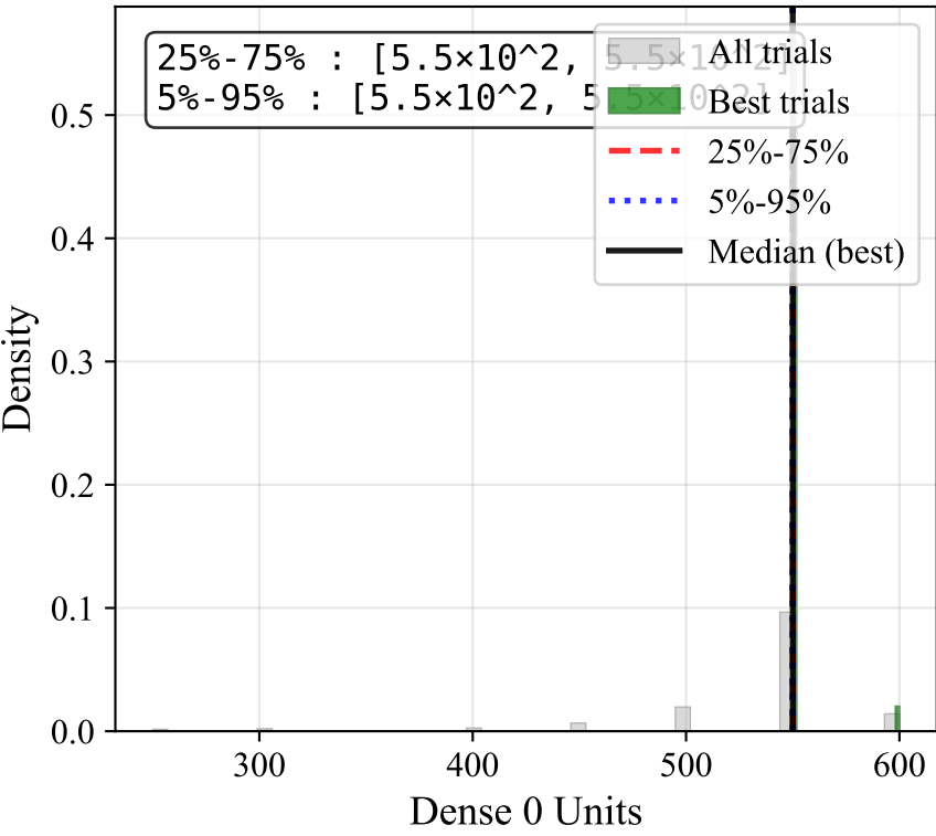
Dense 0 Units
