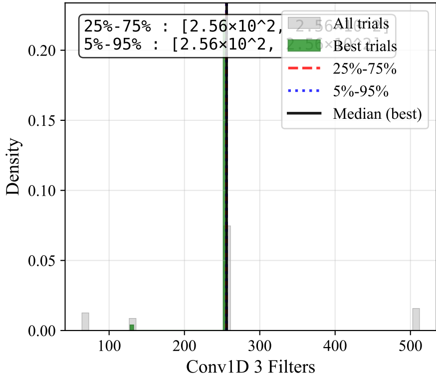
Conv1D 3 Filters
