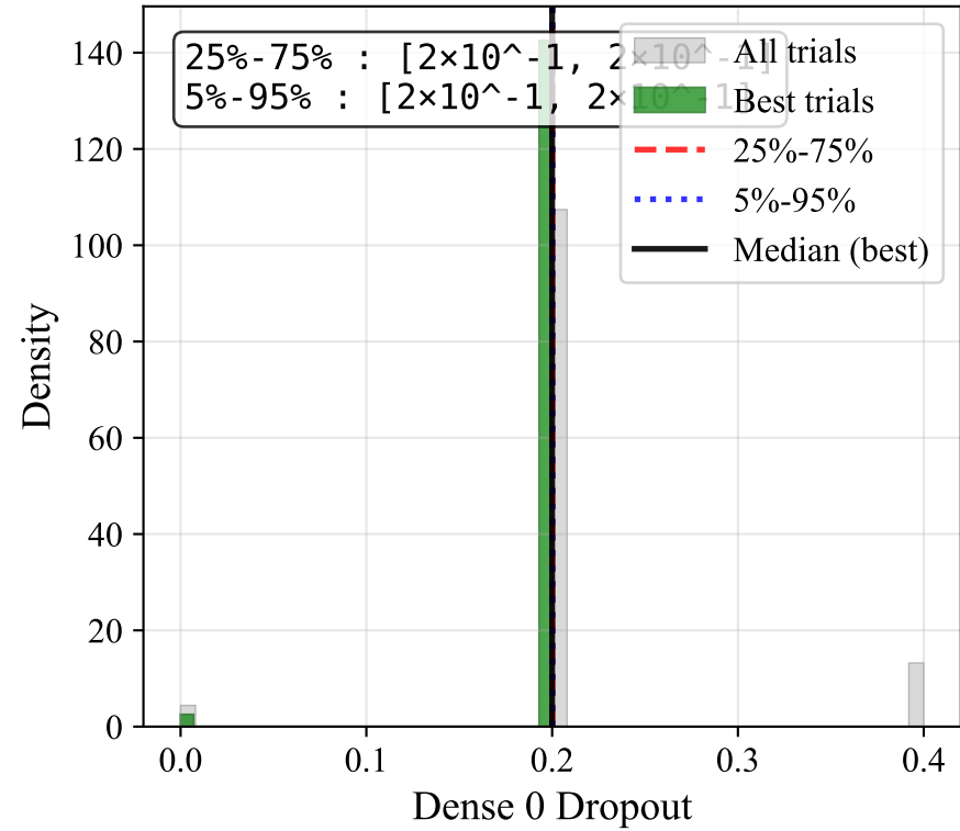
Dense 0 Dropout
