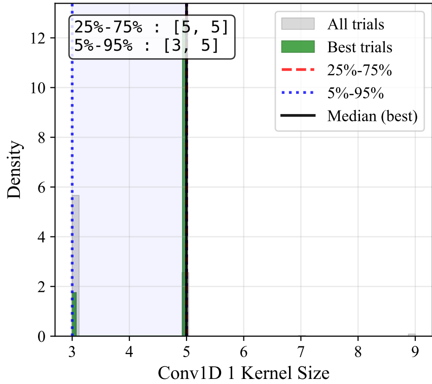
Conv1D 1 Kernel Size
