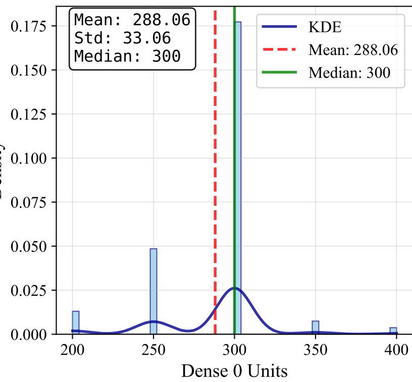
Dense 0 Units
