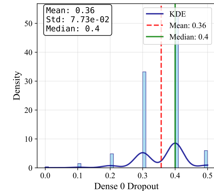
Dense 0 Dropout
