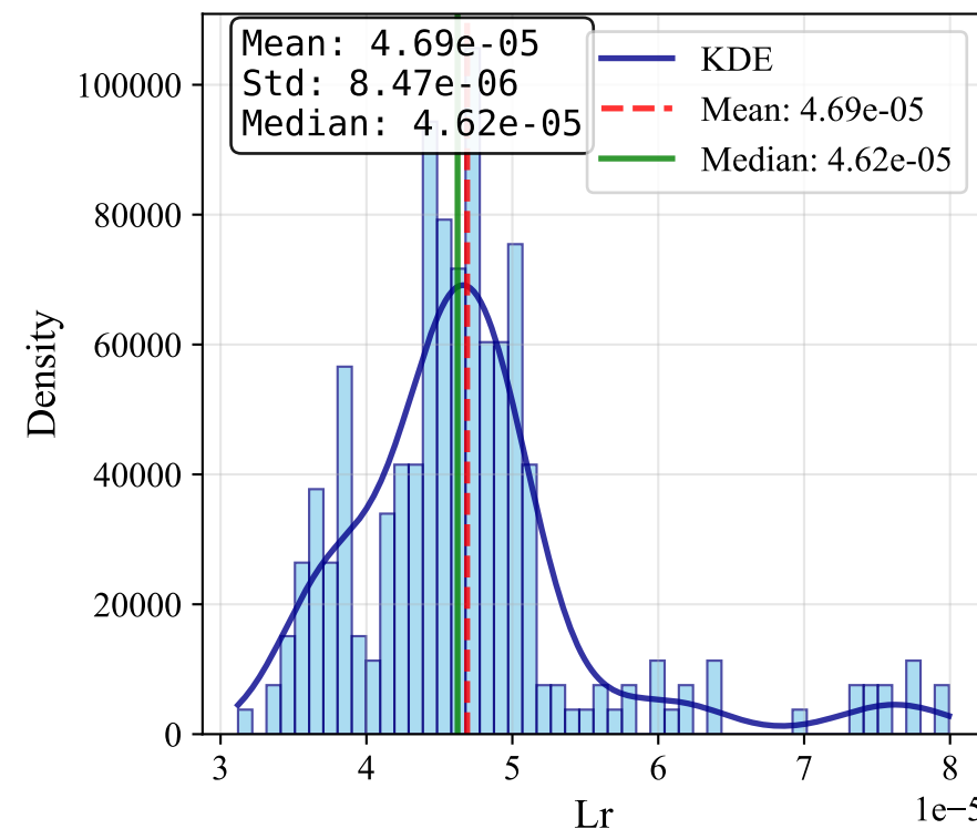
Lr
