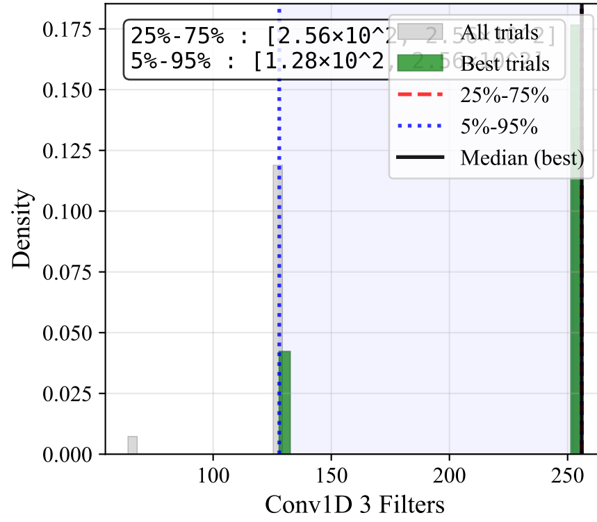
Conv1D 3 Filters
