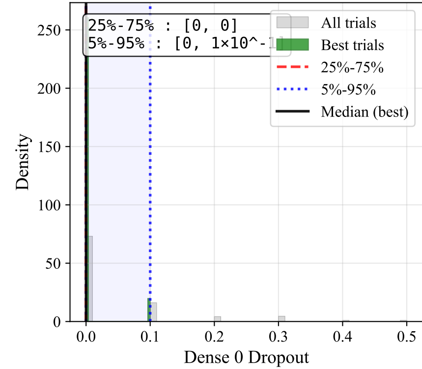
Dense 0 Dropout
