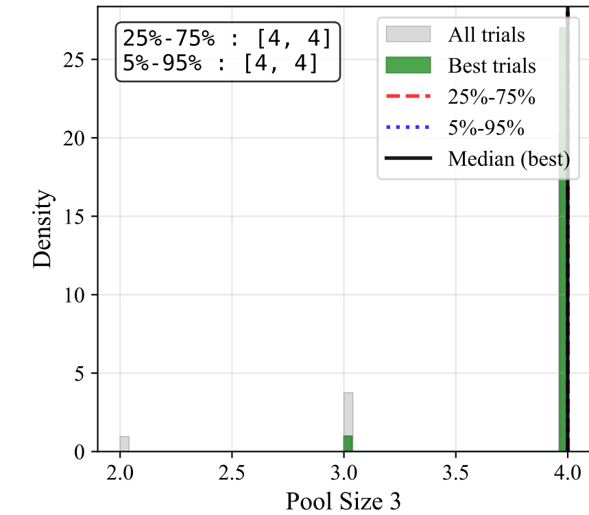
Pool Size 3
