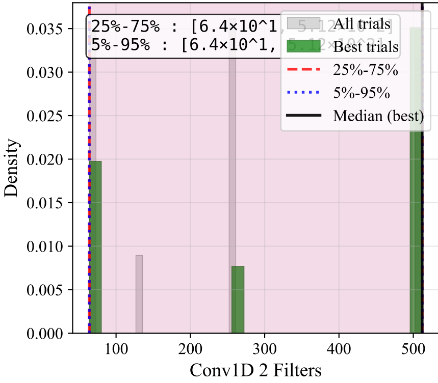
Conv1D 2 Filters
