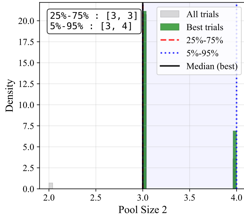
Pool Size 2
