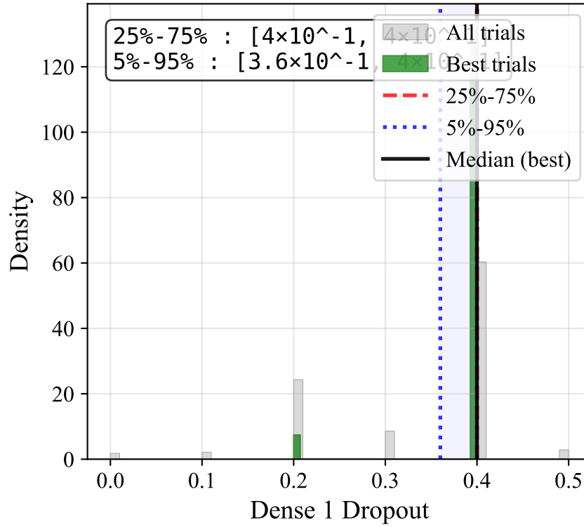
Dense 1 Dropout
