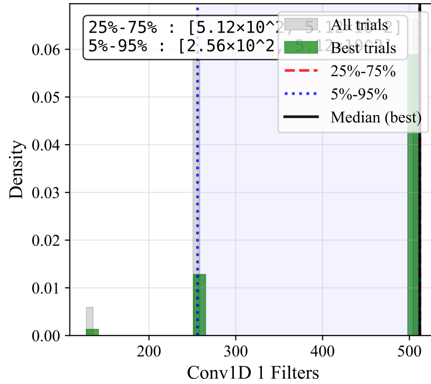
Conv1D 1 Filters
