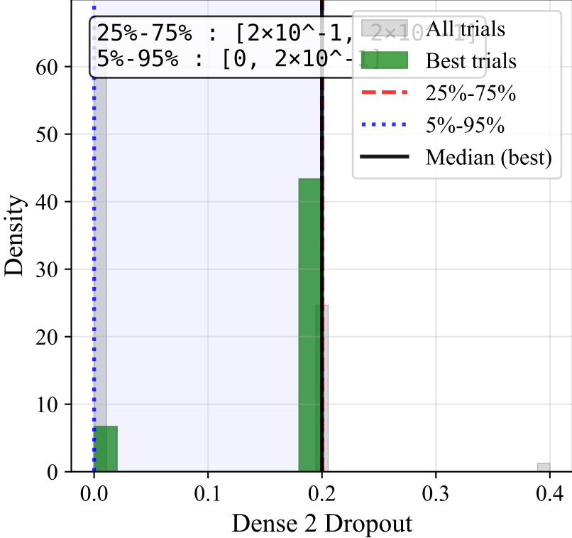
Dense 2 Dropout
