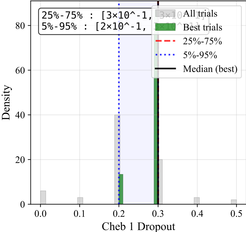
Cheb 1 Dropout
