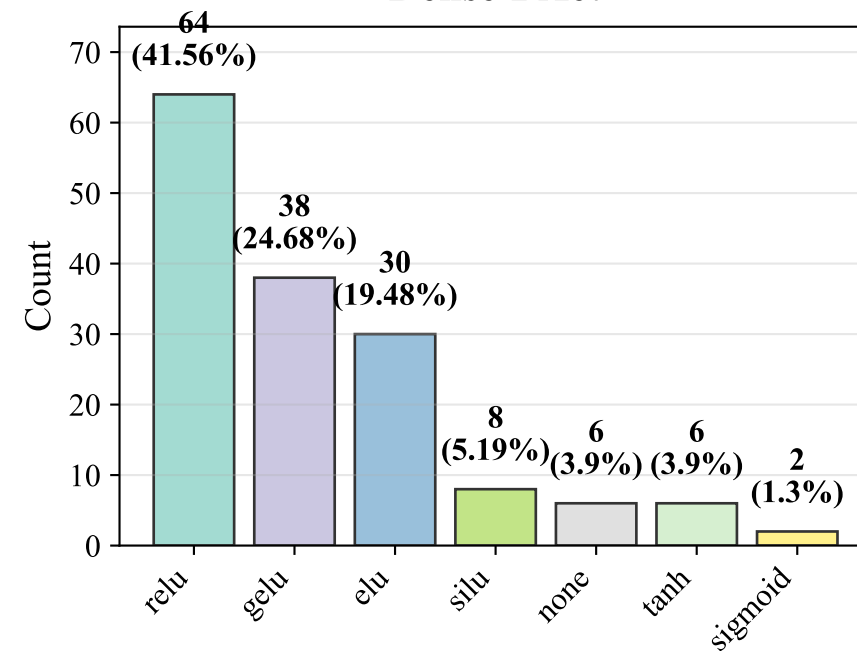
Dense 1 Act
