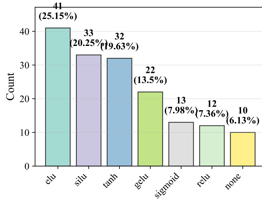
Conv1D 0 Act
