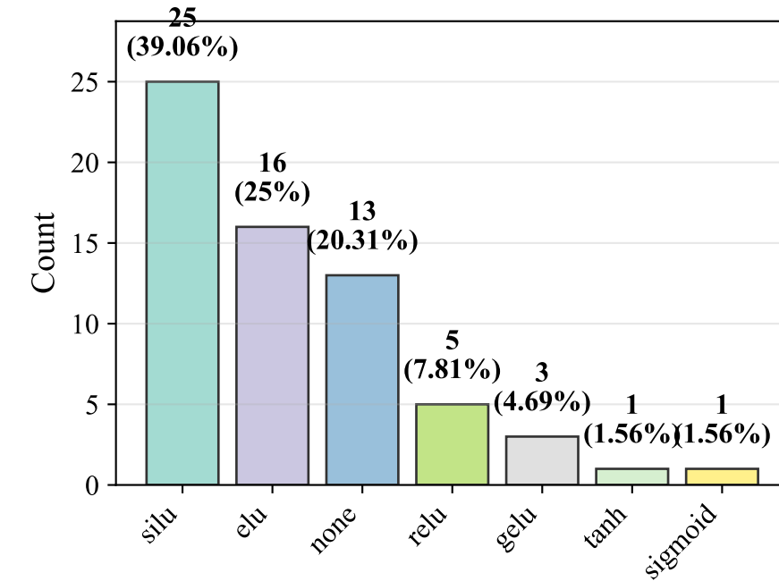
Conv1D 3 Act
