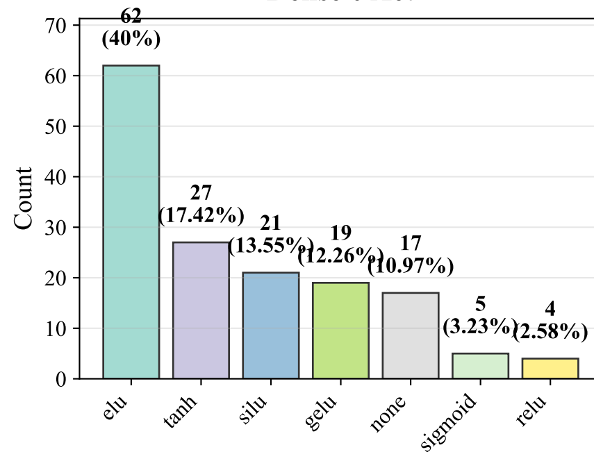
Dense 0 Act
