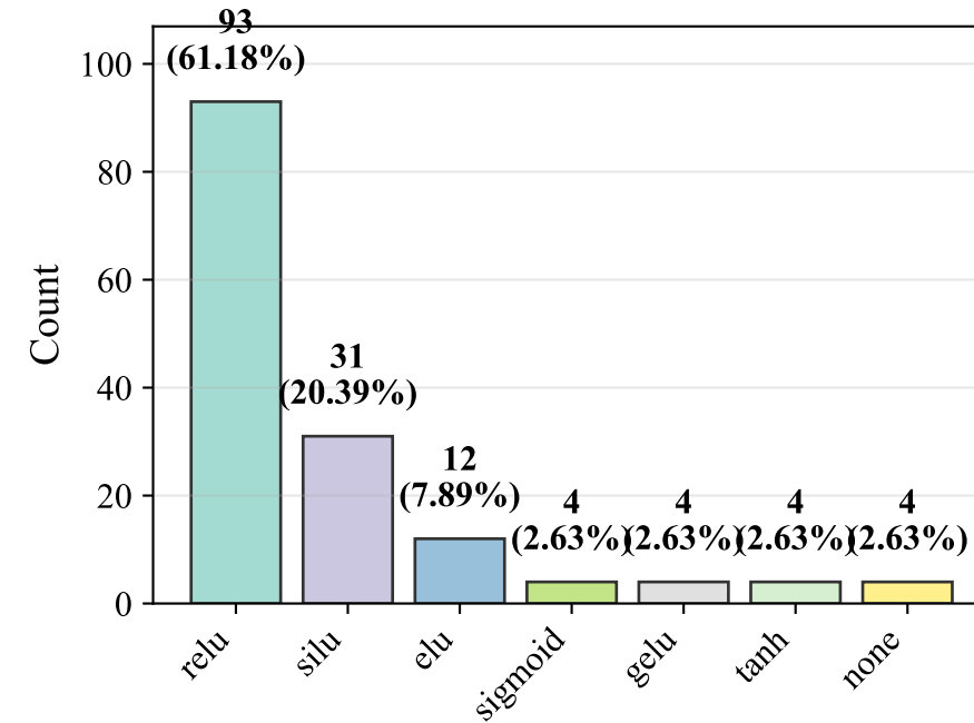
Conv1D 1 Act
