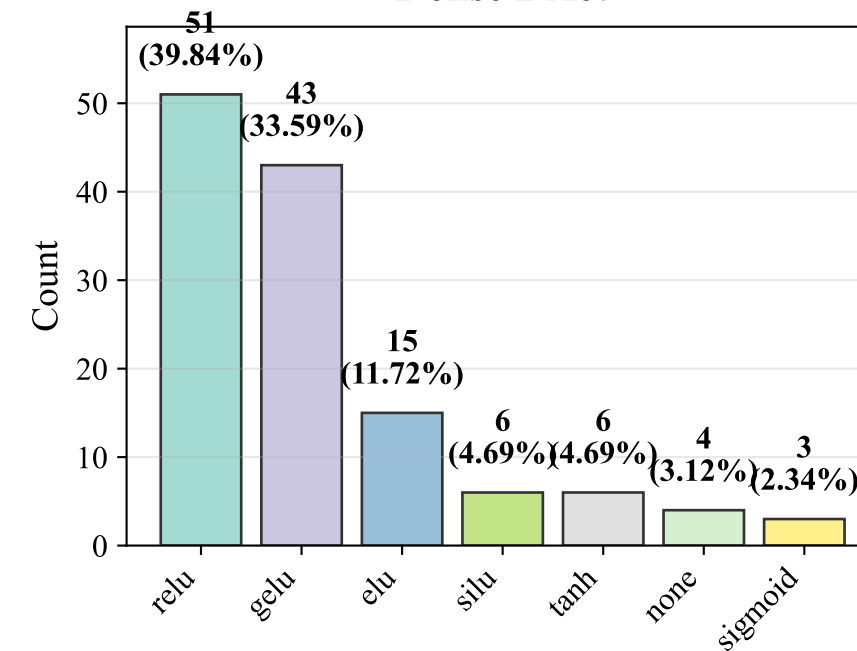
Dense 2 Act
