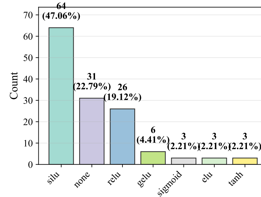
Conv1D 2 Act
