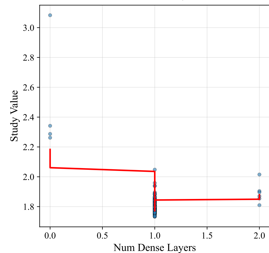
Num Dense Layers
