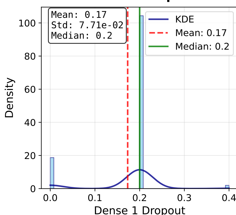
Dense 1 Dropout
