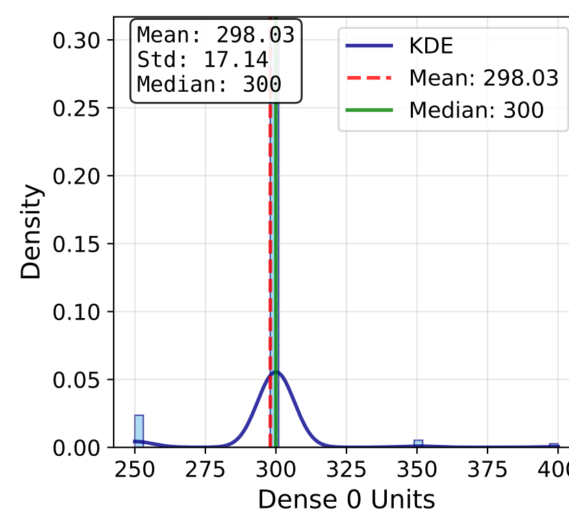
Dense 0 Units
