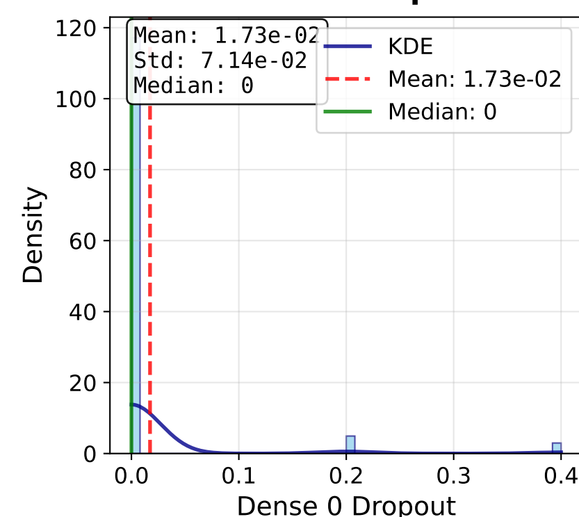
Dense 0 Dropout
