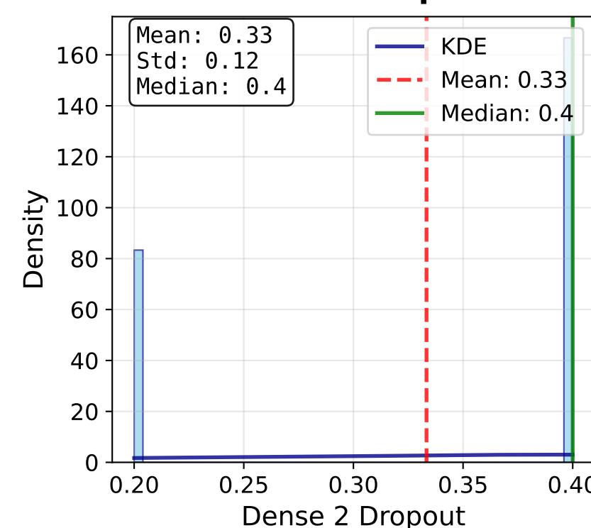
Dense 2 Dropout
