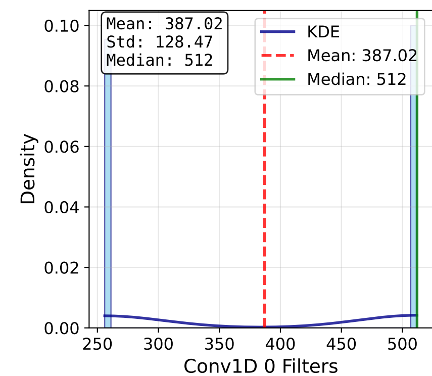
Conv1D 0 Filters
