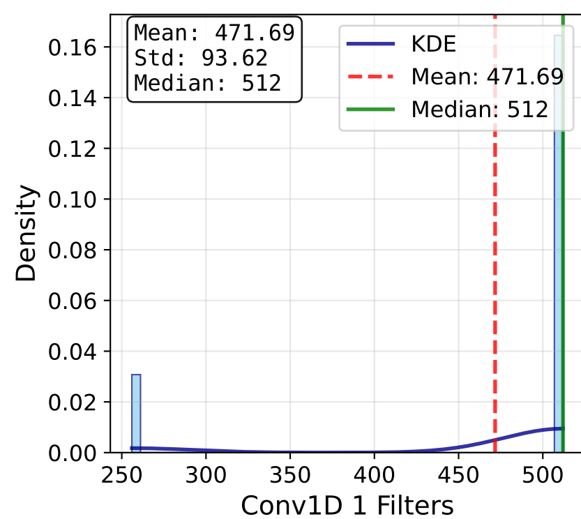
Conv1D 1 Filters
