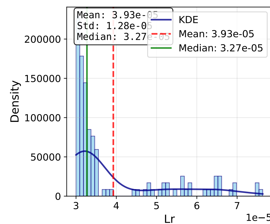
Lr
