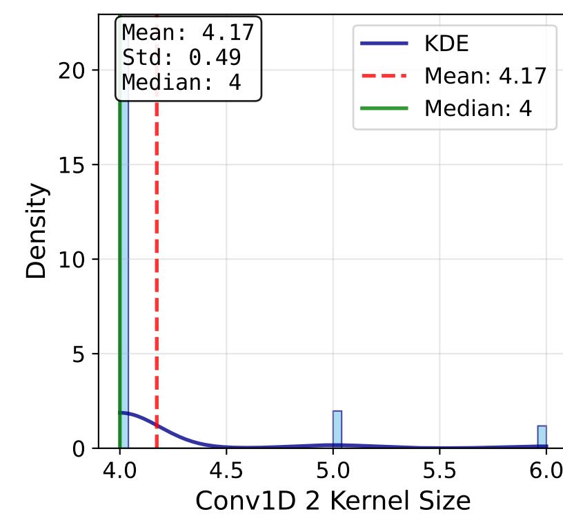
Conv1D 2 Kernel Size
