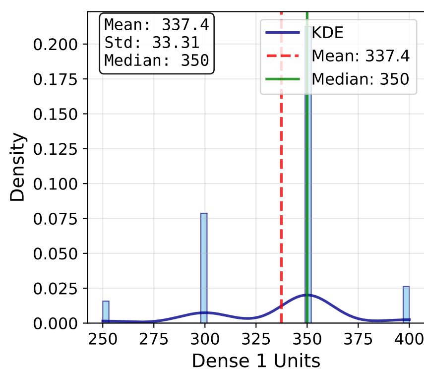
Dense 1 Units
