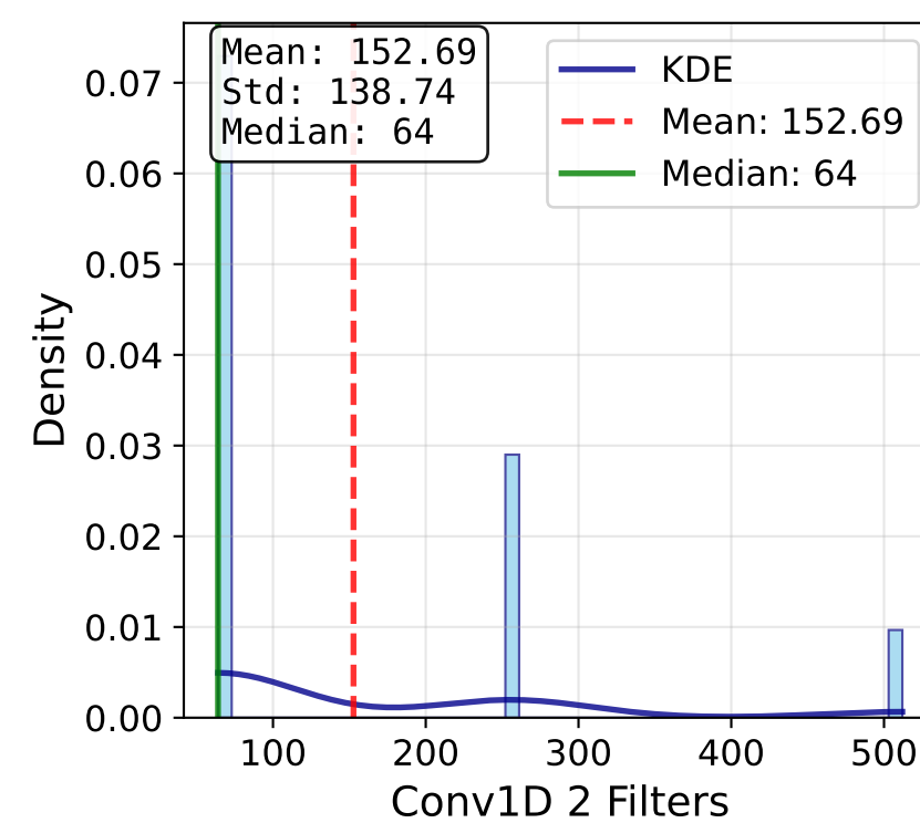
Conv1D 2 Filters
