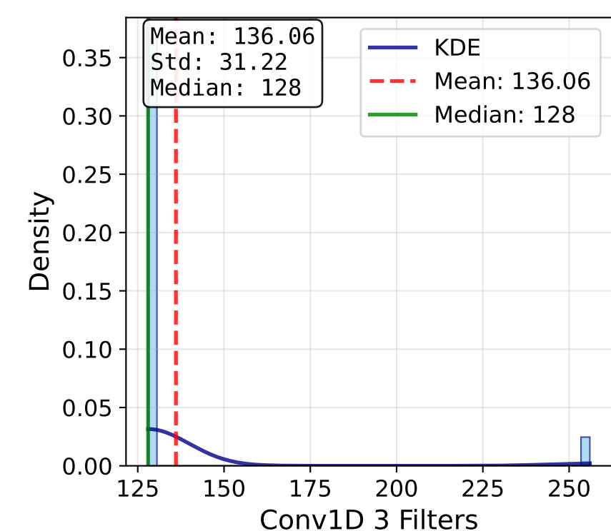
Conv1D 3 Filters
