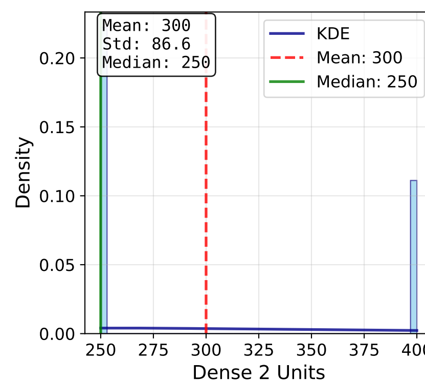
Dense 2 Units
