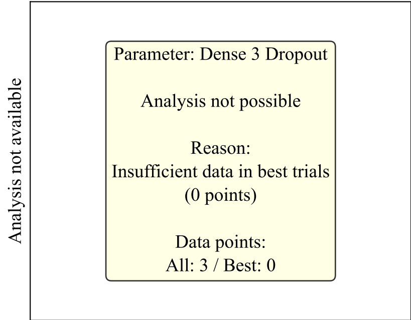
Dense 3 Dropout
