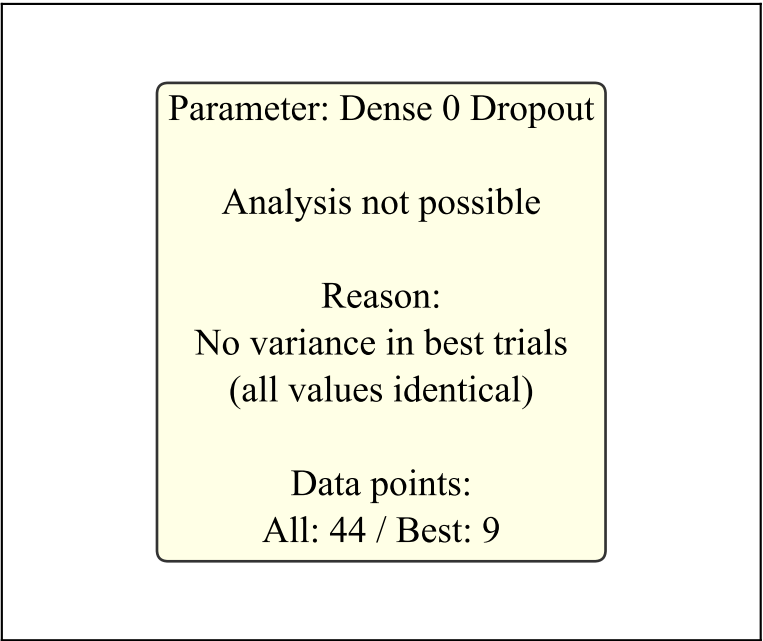
Dense 0 Dropout
