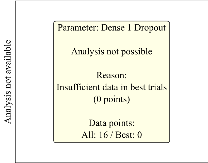
Dense 1 Dropout
