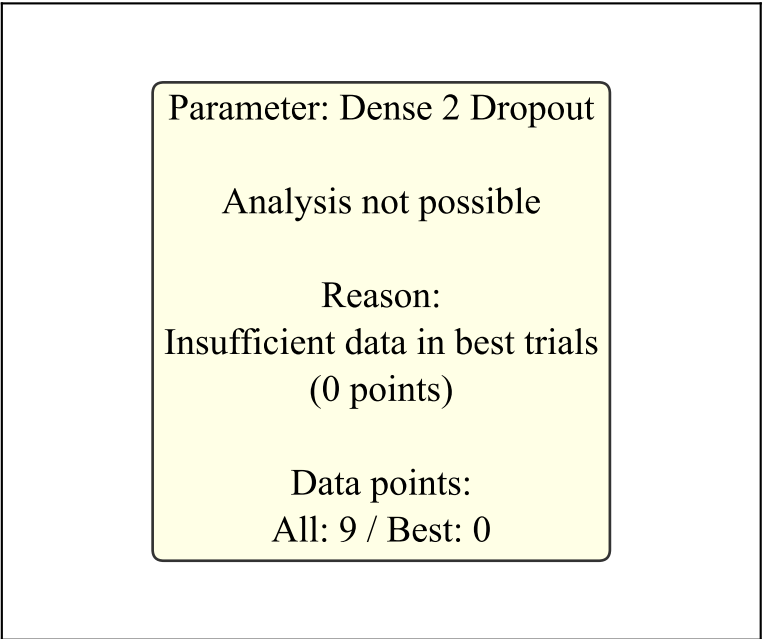
Dense 2 Dropout
