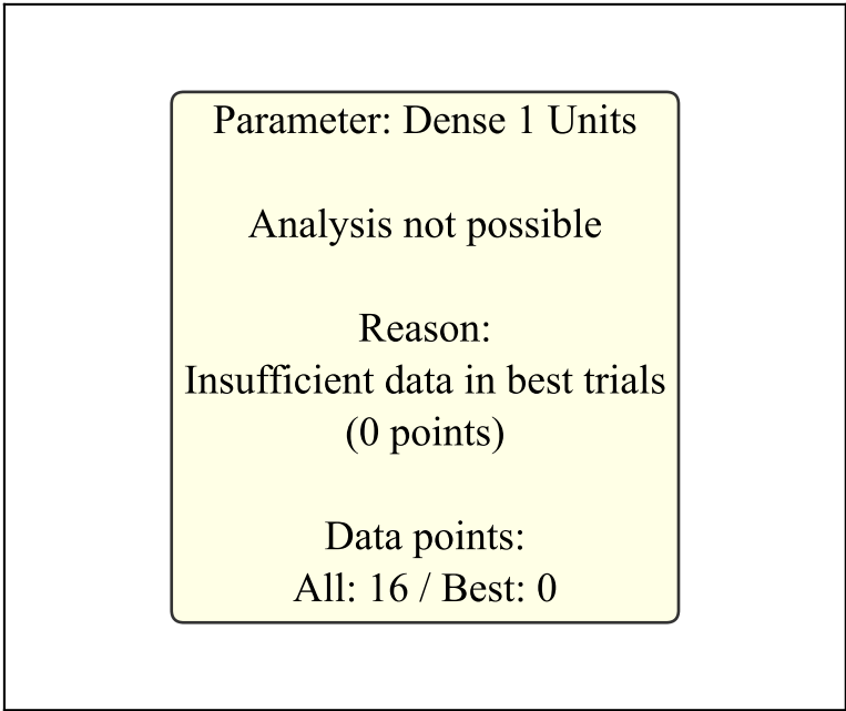
Dense 1 Units
