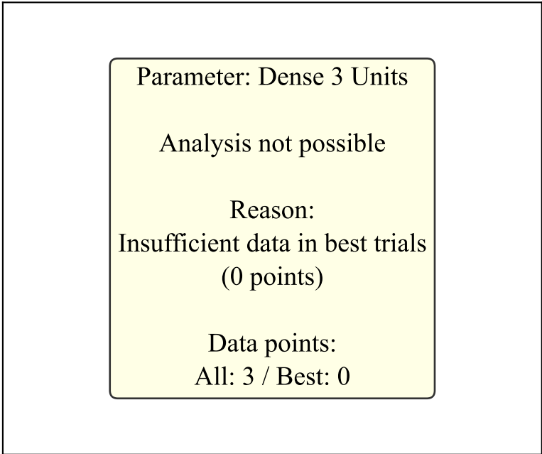
Dense 3 Units
