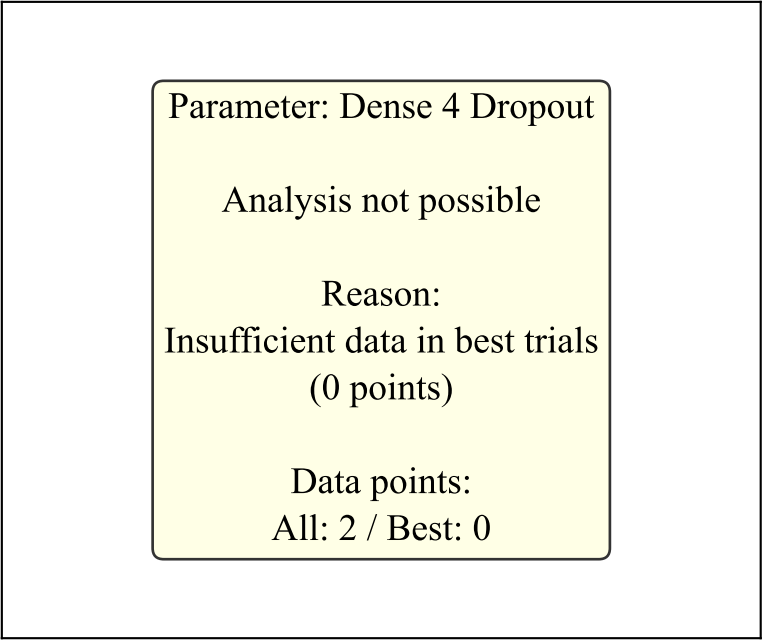
Dense 4 Dropout
