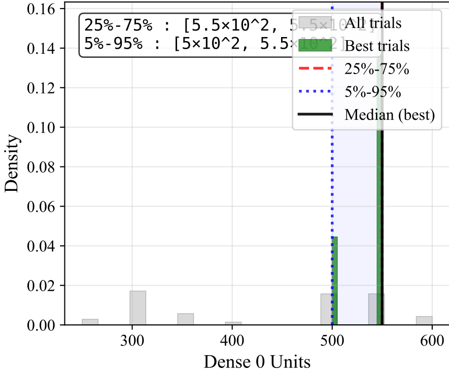
Dense 0 Units
