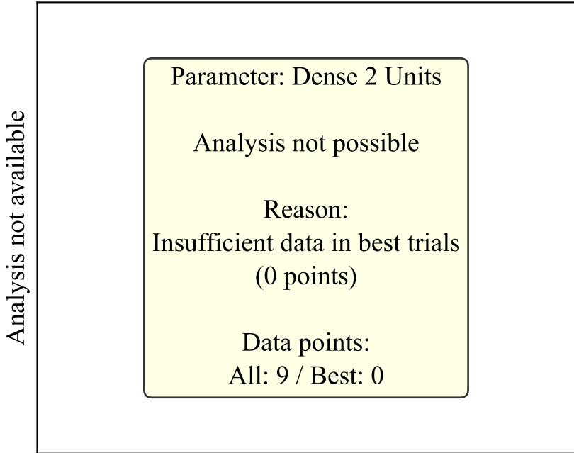
Dense 2 Units
