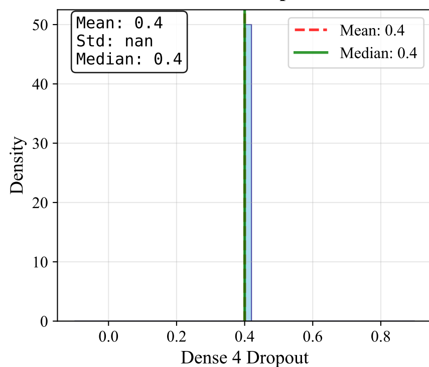
Dense 4 Dropout
