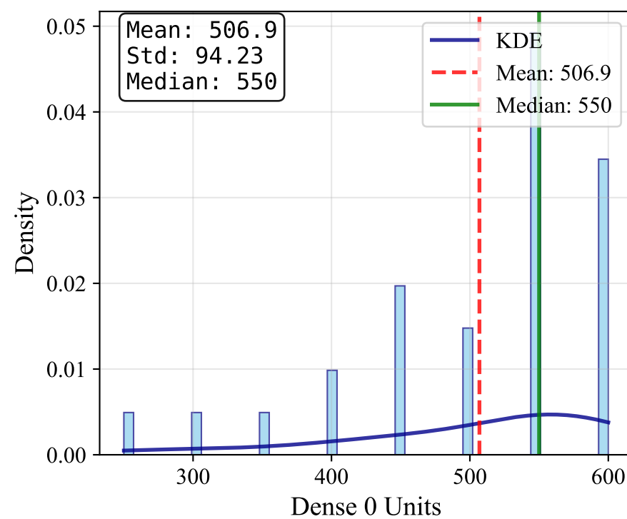
Dense 0 Units
