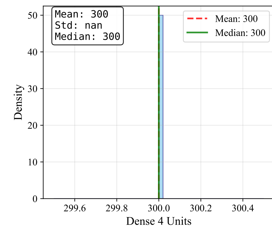
Dense 4 Units
