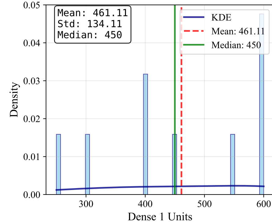
Dense 1 Units
