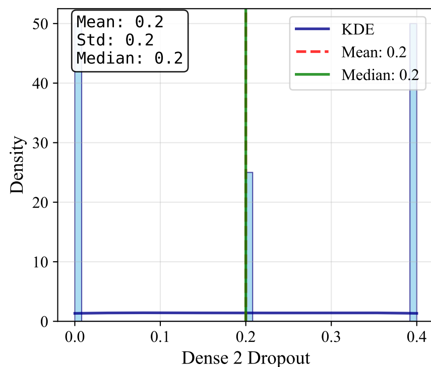
Dense 2 Dropout
