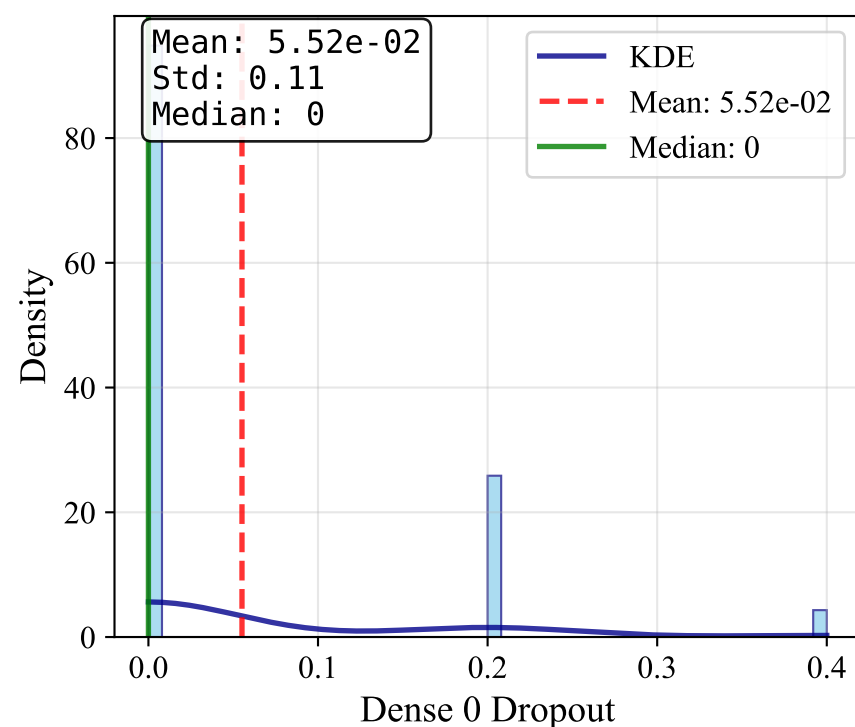
Dense 0 Dropout
