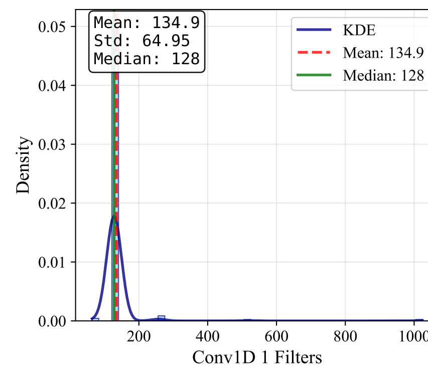
Conv1D 1 Filters
