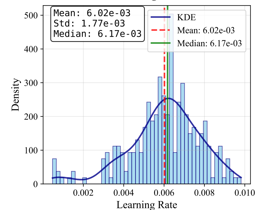
Learning Rate
