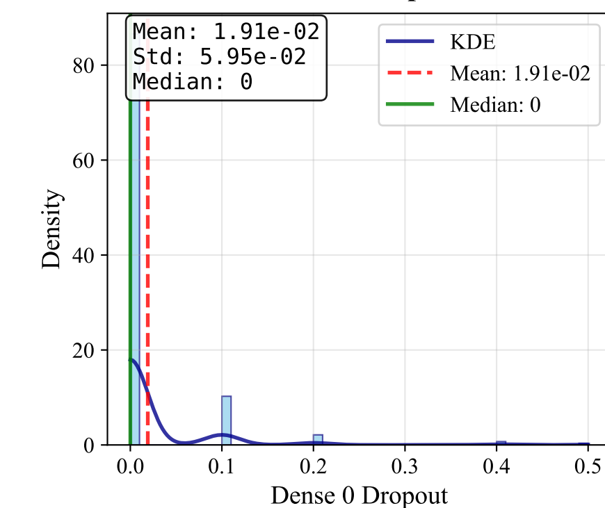
Dense 0 Dropout
