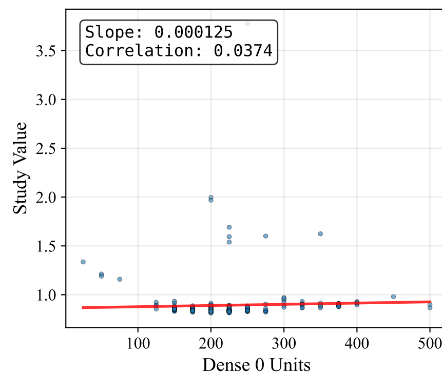
Dense 0 Units
