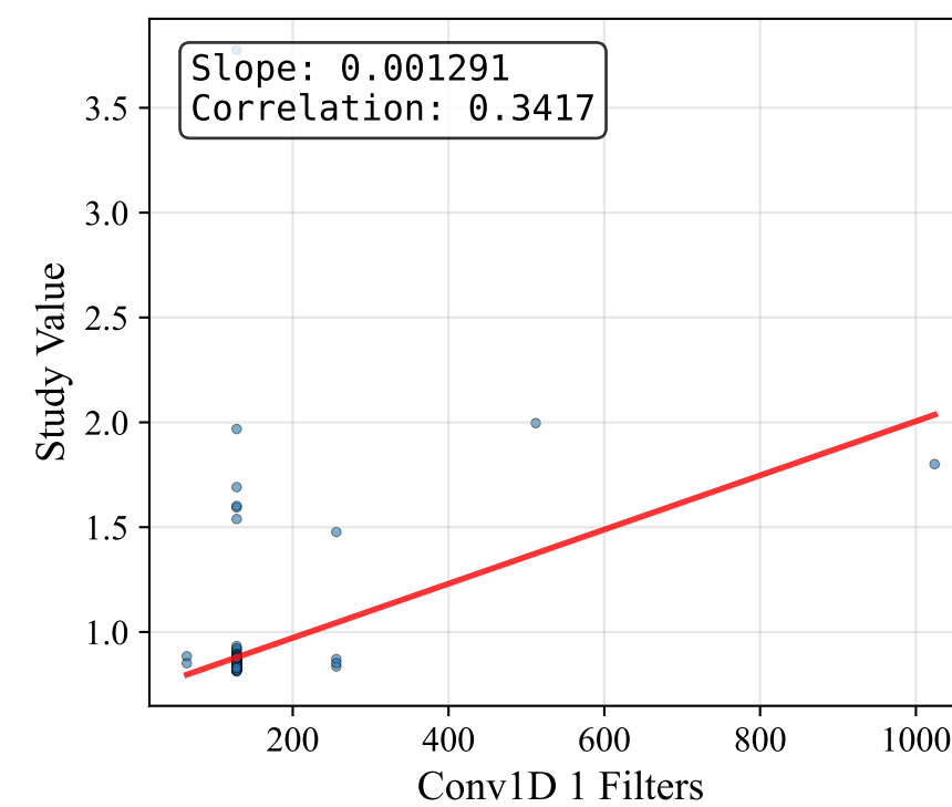
Conv1D 1 Filters
