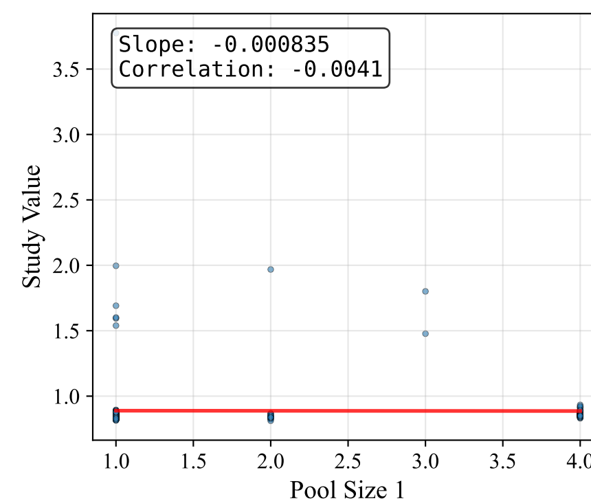
Pool Size 1
