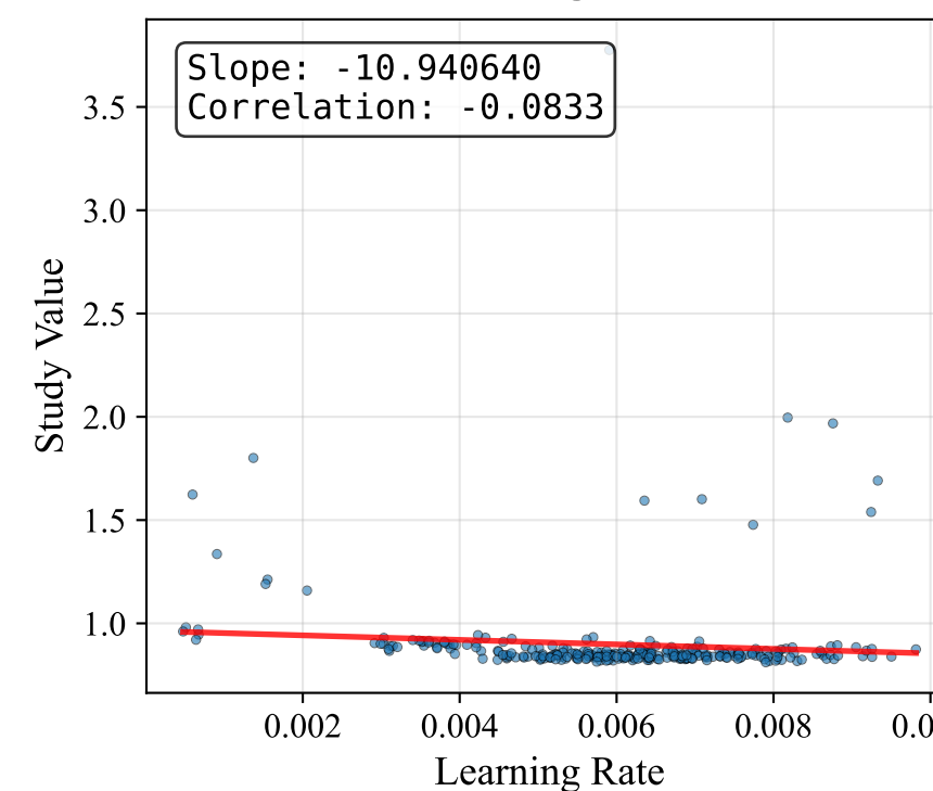
Learning Rate
