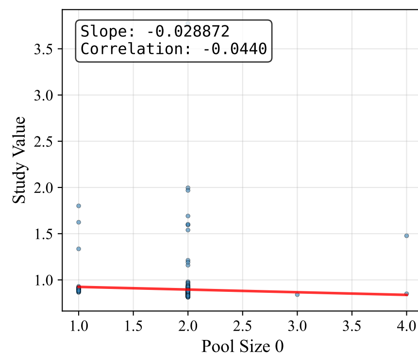
Pool Size 0
