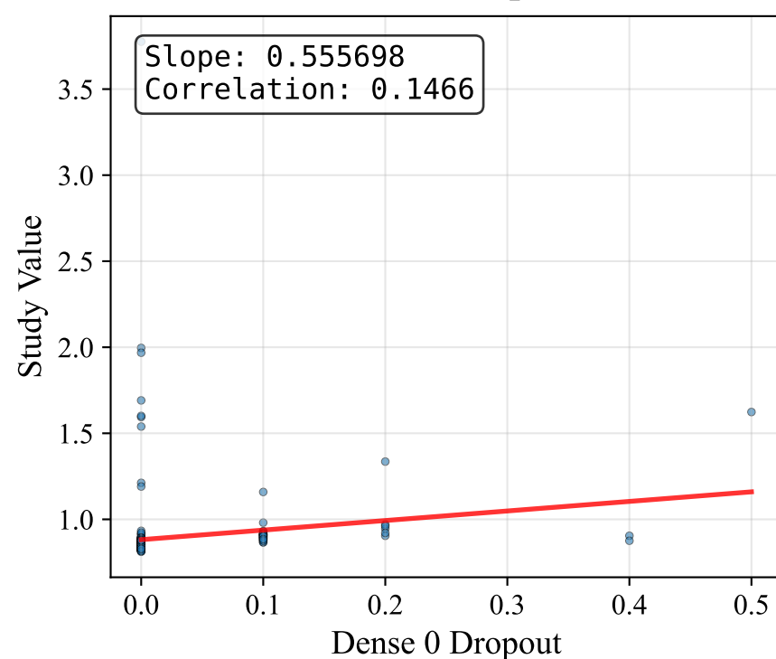
Dense 0 Dropout
