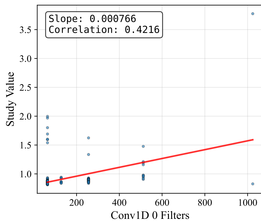
Conv1D 0 Filters
