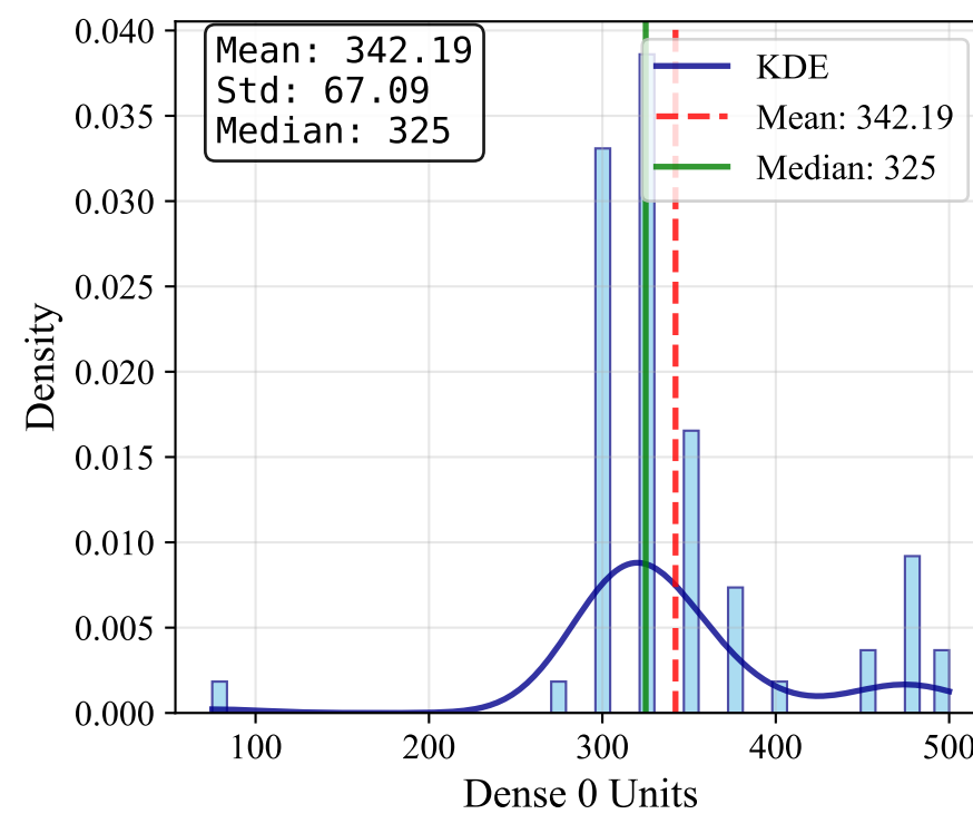
Dense 0 Units
