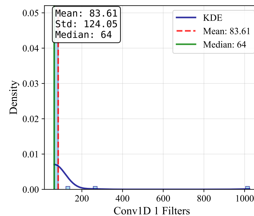
Conv1D 1 Filters
