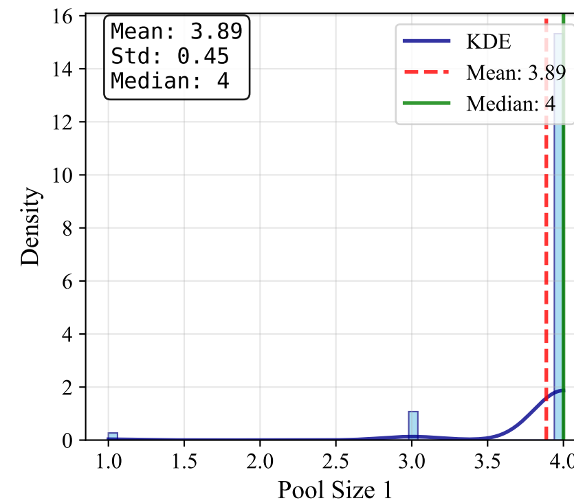
Pool Size 1
