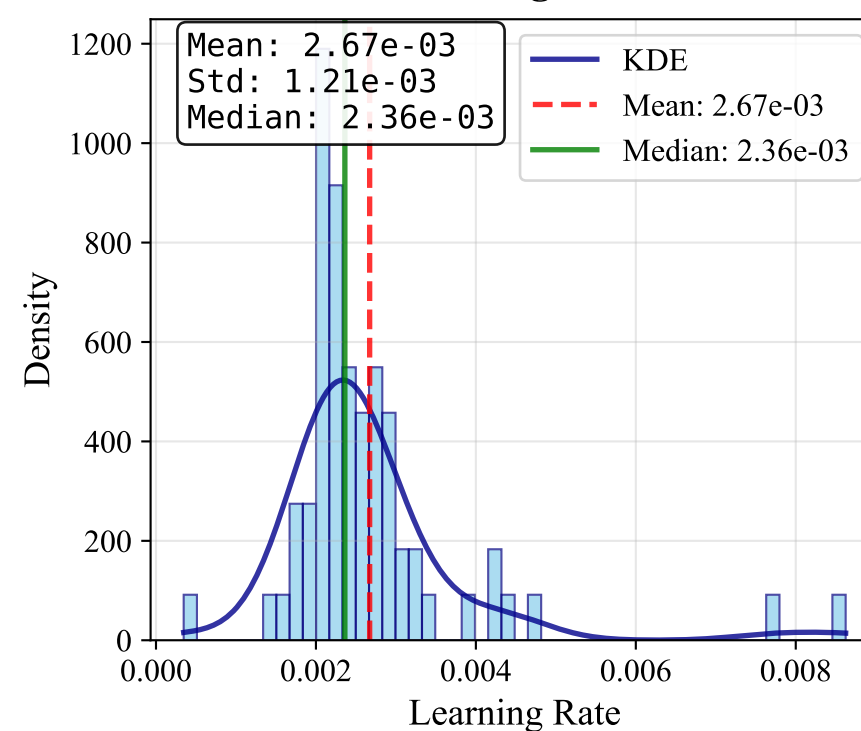
Learning Rate
