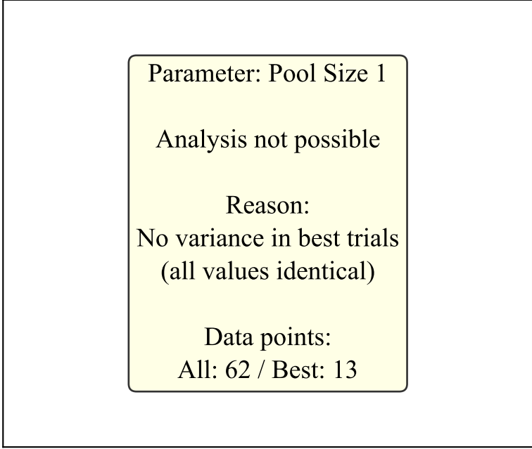
Pool Size 1
