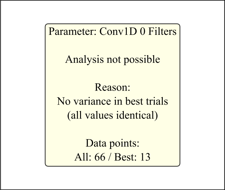
Conv1D 0 Filters
