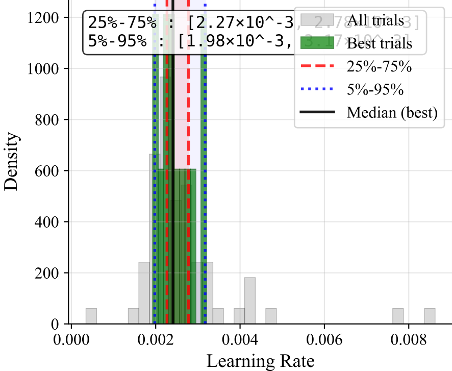
Learning Rate
