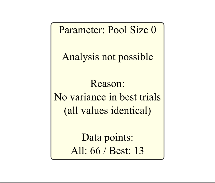
Pool Size 0
