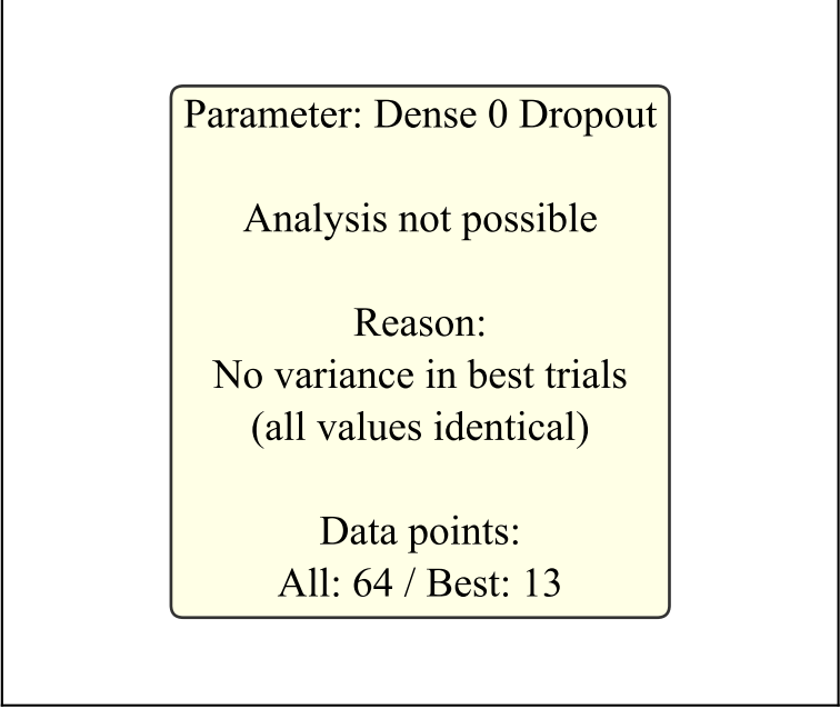
Dense 0 Dropout
