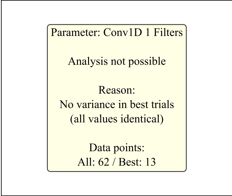
Conv1D 1 Filters
