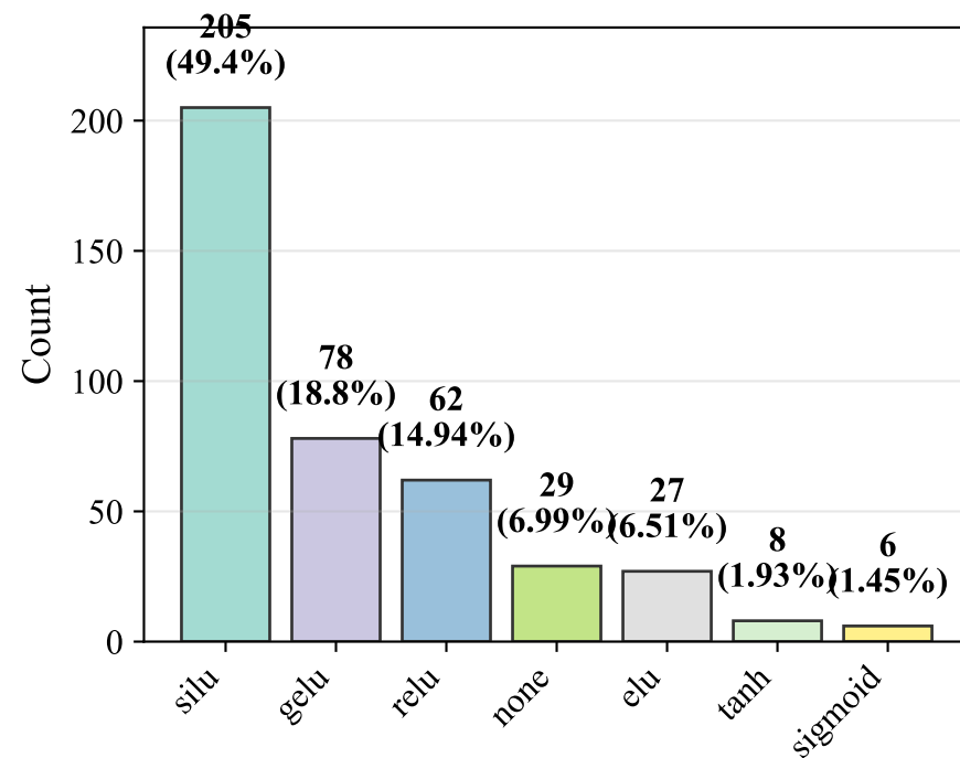
Conv2D 0 Act
