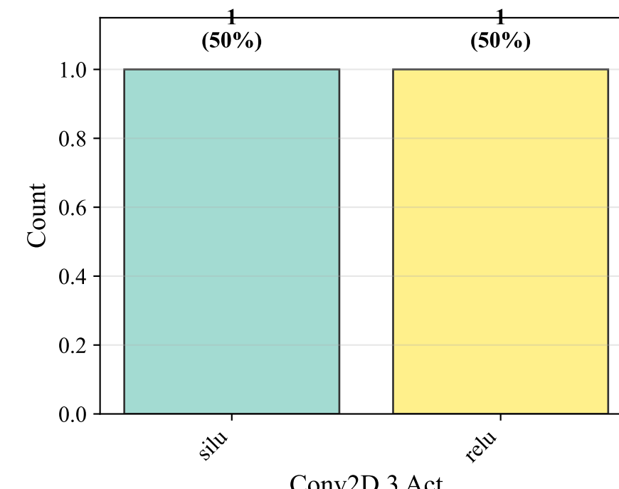
Conv2D 3 Act
