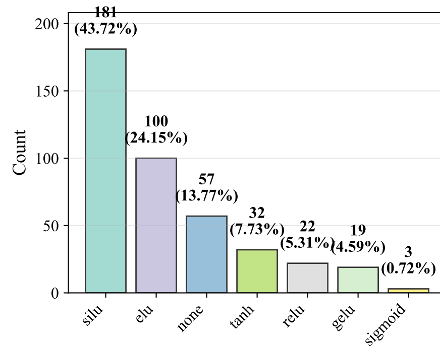
Conv2D 1 Act
