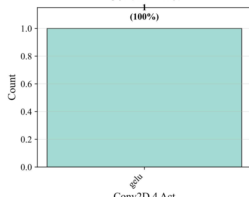
Conv2D 4 Act
