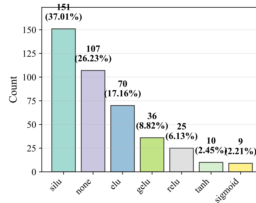
Conv2D 2 Act
