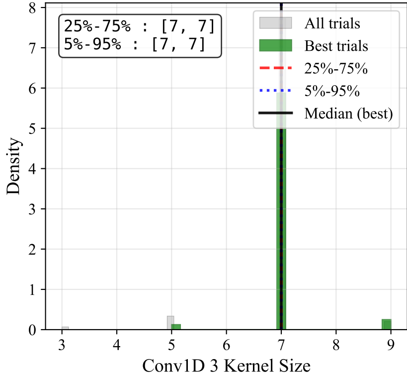
Conv1D 3 Kernel Size
