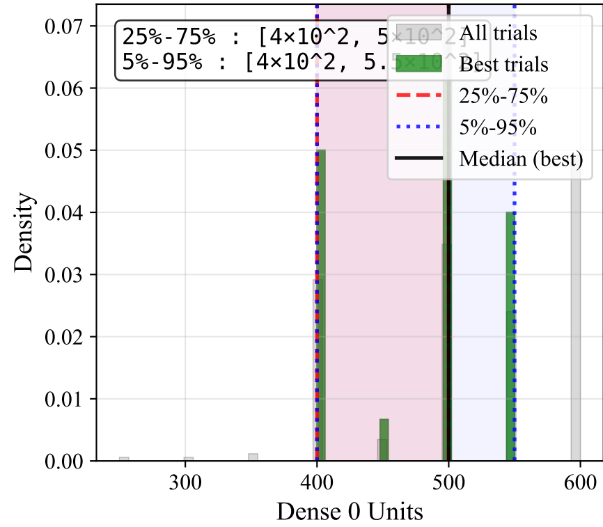
Dense 0 Units
