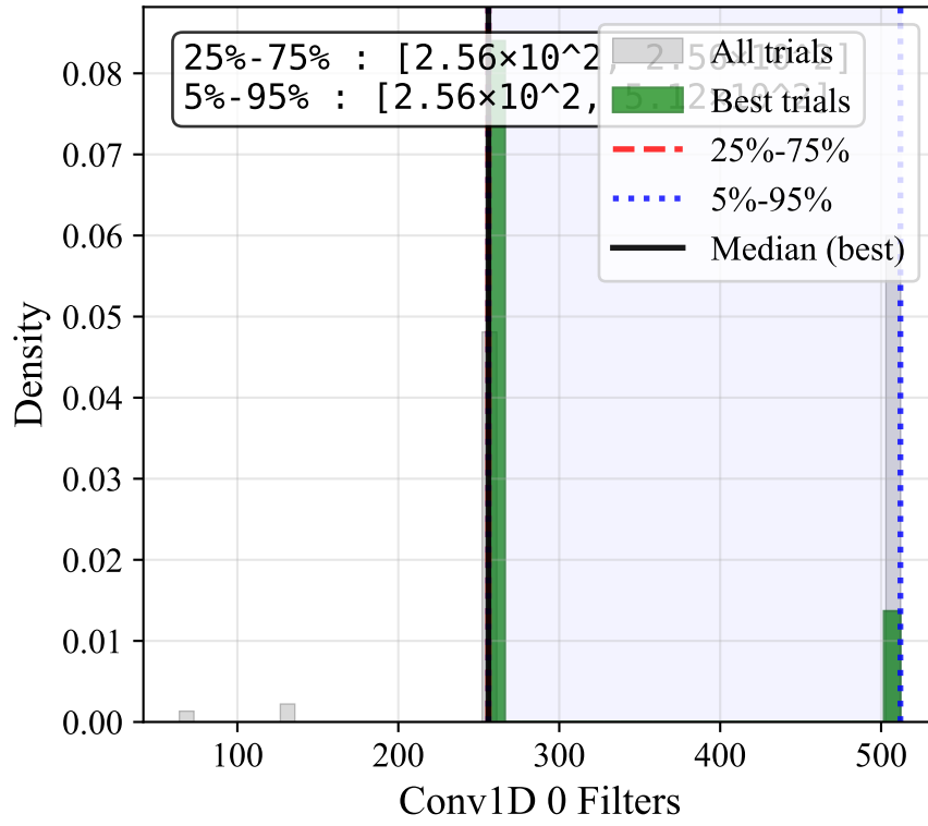
Conv1D 0 Filters
