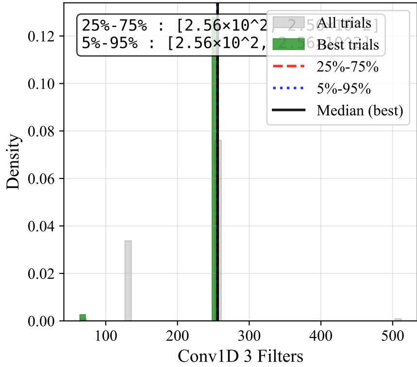
Conv1D 3 Filters
