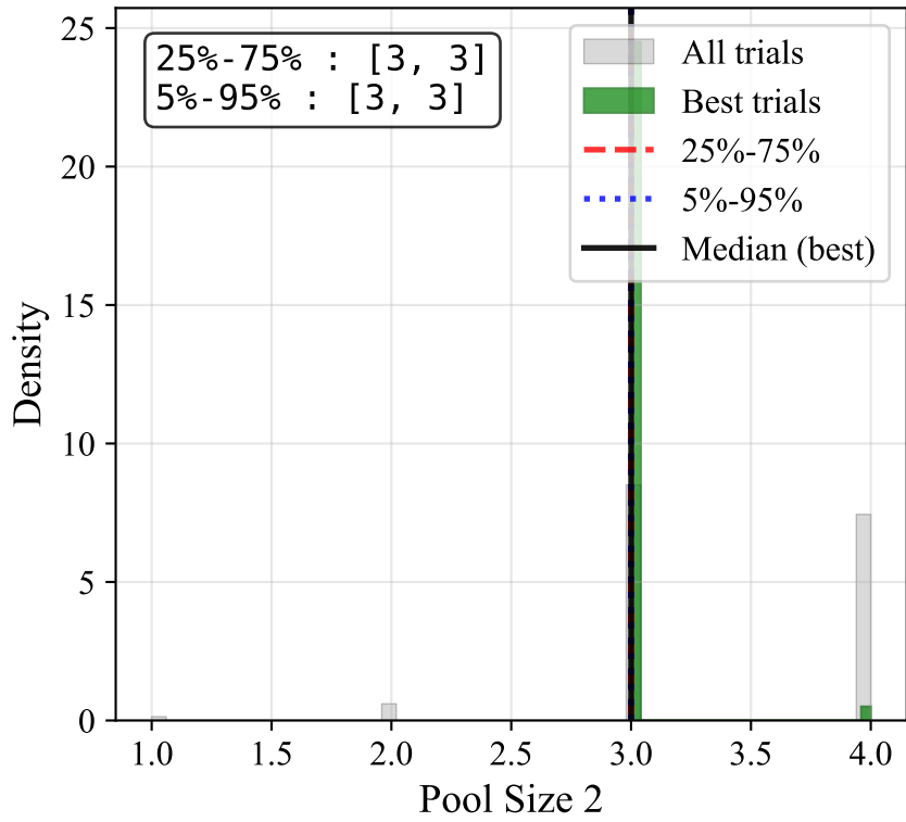
Pool Size 2
