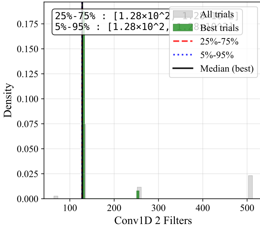
Conv1D 2 Filters
