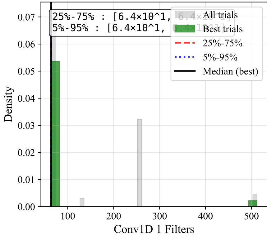
Conv1D 1 Filters
