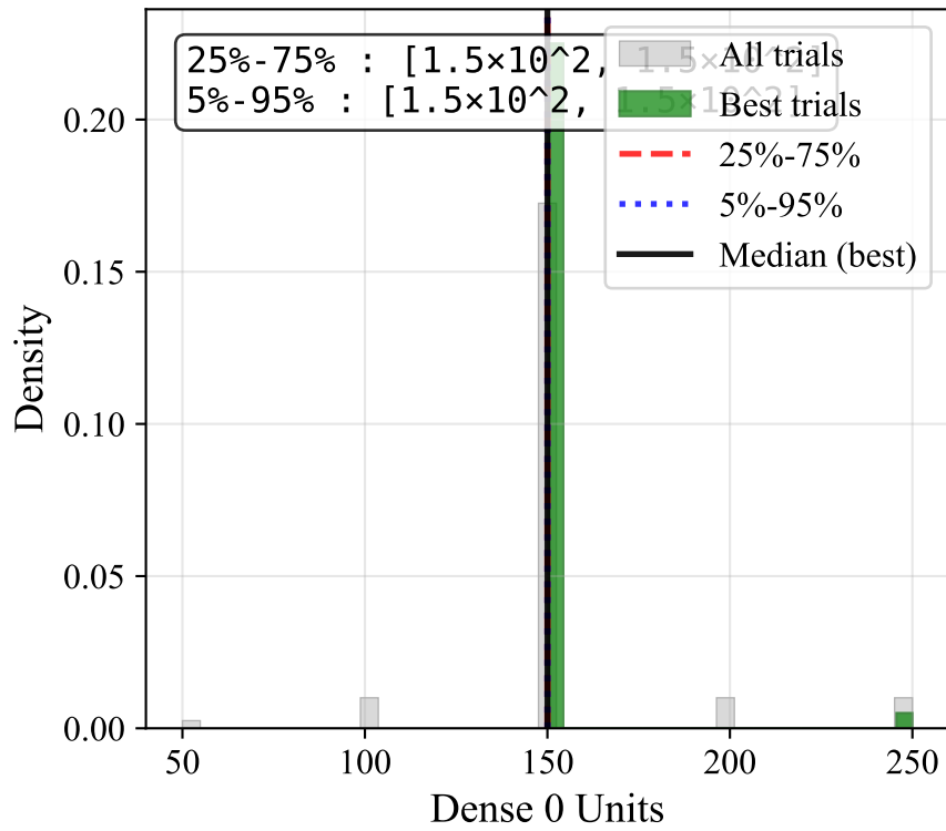
Dense 0 Units
