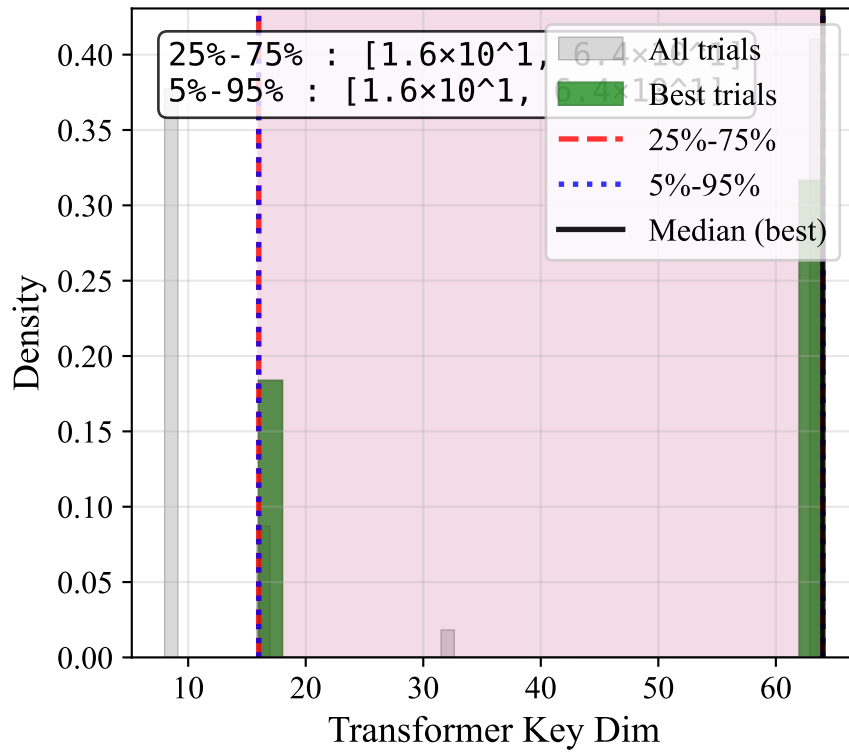
Transformer Key Dim
