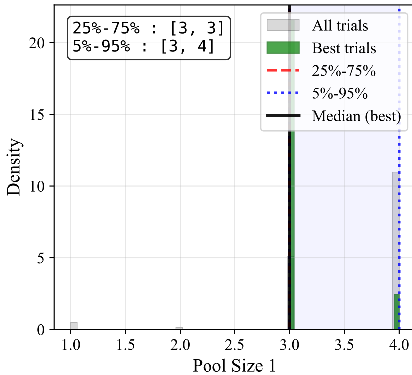
Pool Size 1
