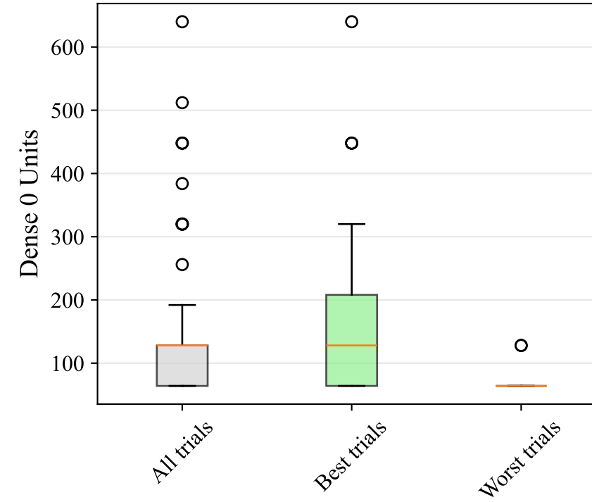
Dense 0 Units
