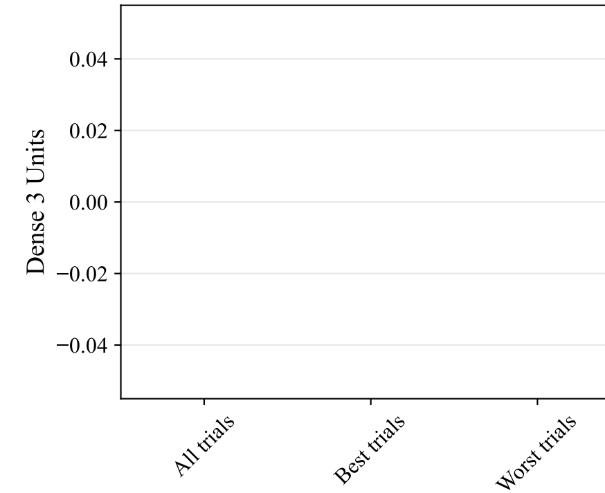
Dense 3 Units
