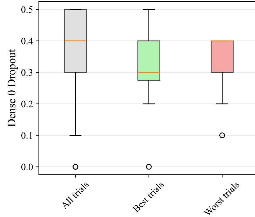
Dense 0 Dropout
