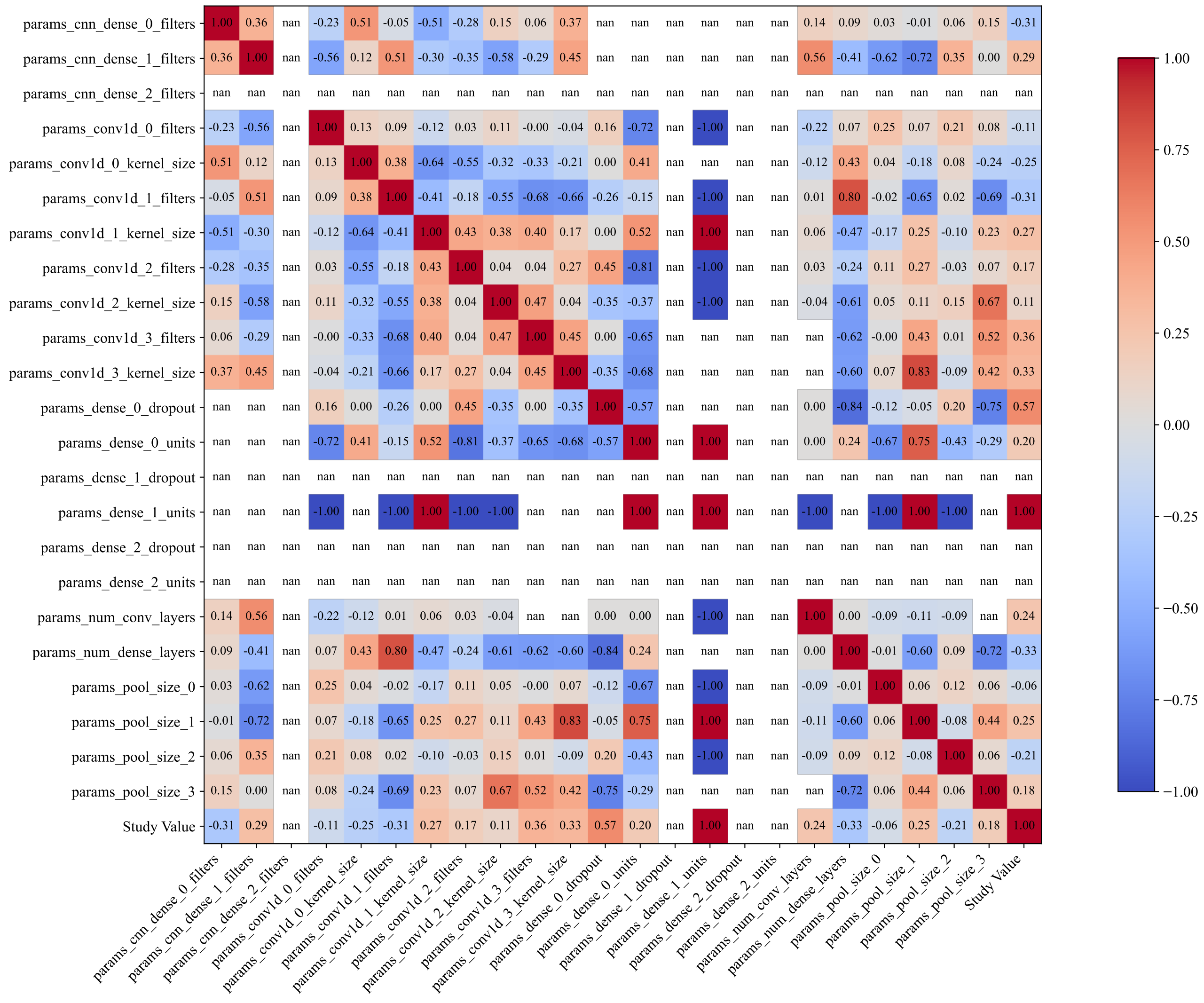
SpearmanCorrelation
